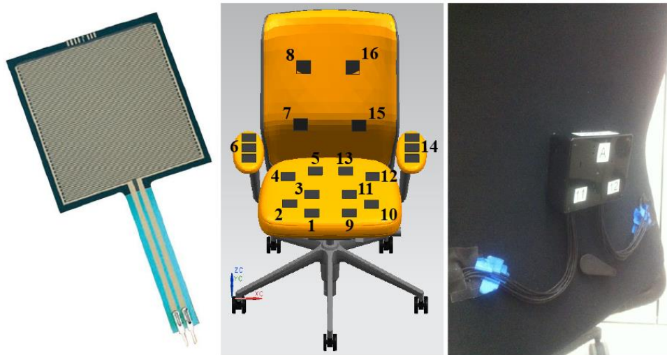
5 Figure A1: Left: A pressure sensor (FSR® 406); middle: Sensor distribution on the seat pan, on the backrest and on the armrests of the office chair. Sensors were numbered from one to 16; right: Box with a Motion-Module (accelerometer, gyroscope and magnetometer) fixed to the backrest of the office chair.
