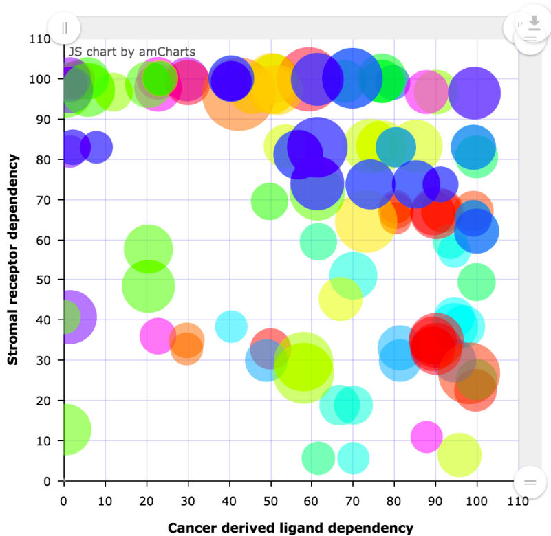
Cancer cell-ligand → Stromal receptor
