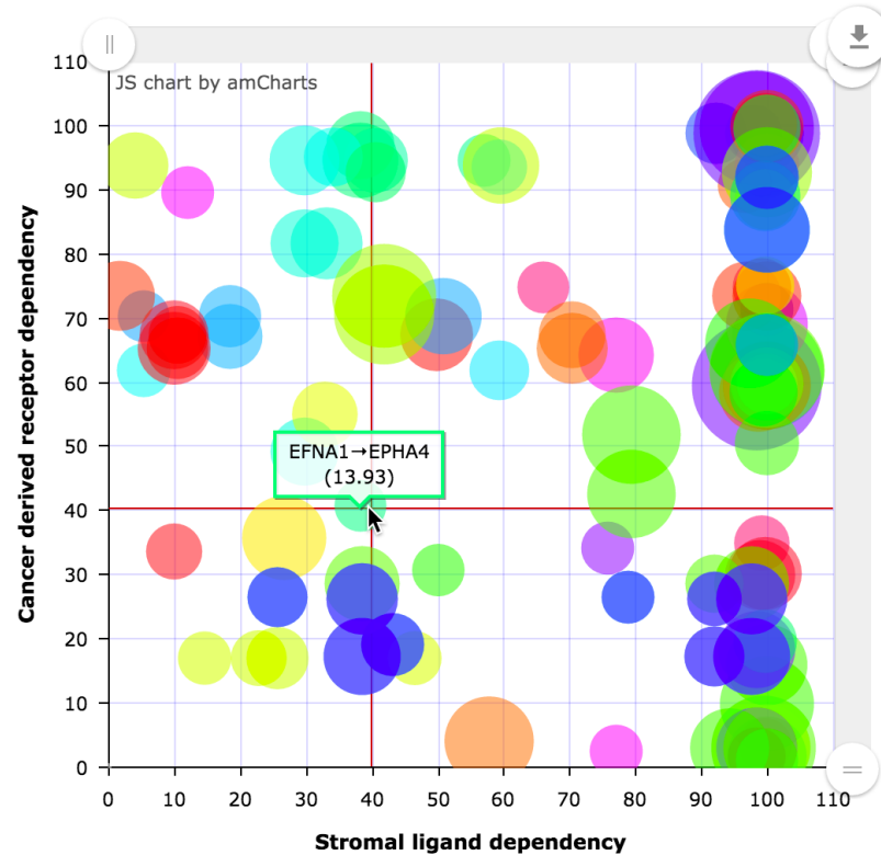
Stromal ligand → Cancer cell-receptor
