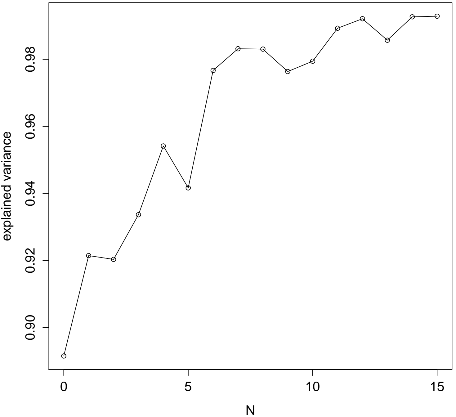
explained variance,from N=0 to N=15
