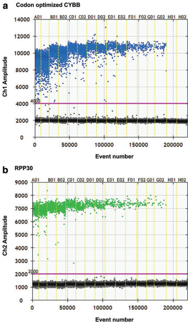
Supplementary Figure S3. Concomitant reduction in codon-optimized CYBB and RPP30 concentration after dilution of template gDNA with water. In this experiment, water was used to dilute template gDNA. (a) Blue dots indicate positive droplets for CO CYBB . (b) Green dots indicate positive droplets for RPP30 . Black dots indicate negative droplets. Letters A to G indicate the amount of template present from 32 ng down to 0.125 ng. The pink line represents the threshold for discriminating droplets.
