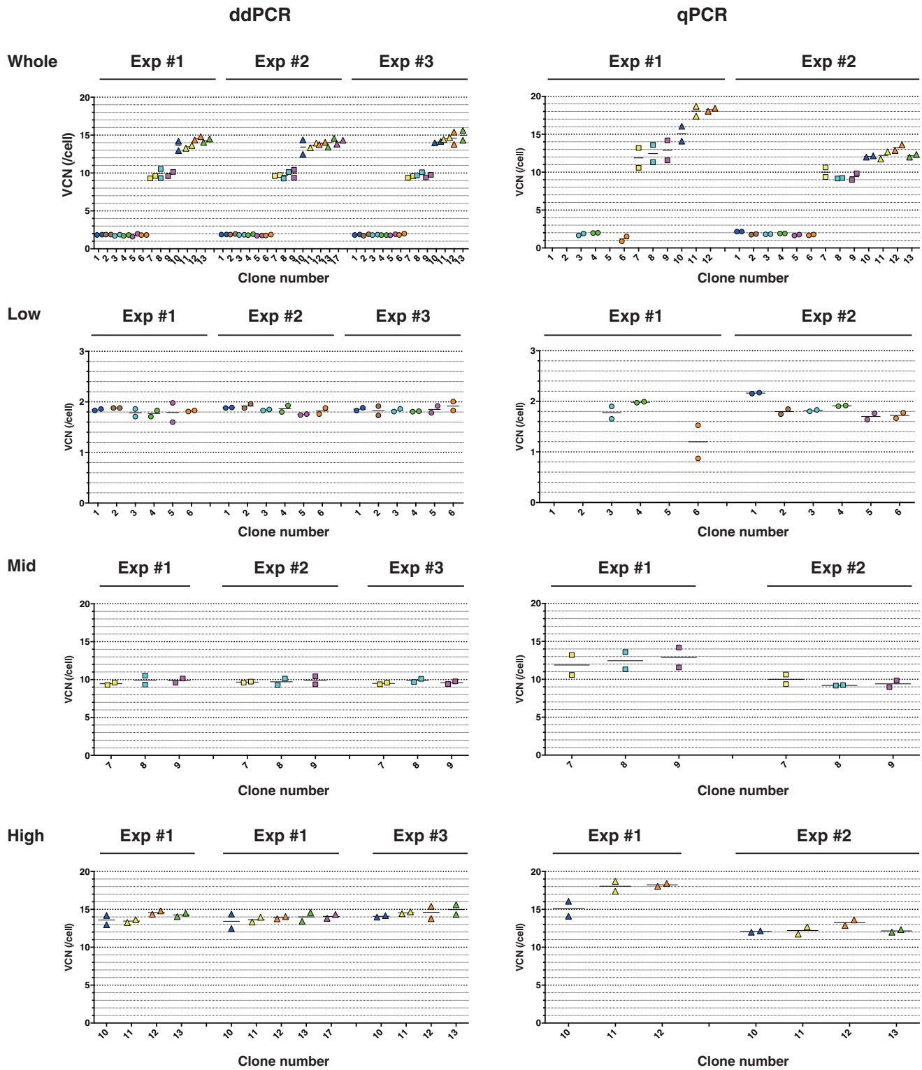
Supplementary Figure S5. Combined side-by-side comparison of VCN estimation between ddPCR and qPCR. Shown are the combined VCN estimation results obtained in this study by either ddPCR (three experiments) or qPCR (two experiments). Clones from the low, mid, or high categories were analyzed. Each clone is represented by the same-shaped symbol and color. Experiment names (ddPCR Exp #1–#3 and qPCR Exp #1 and #2) are the same as those shown in Supplementary Table S2.
