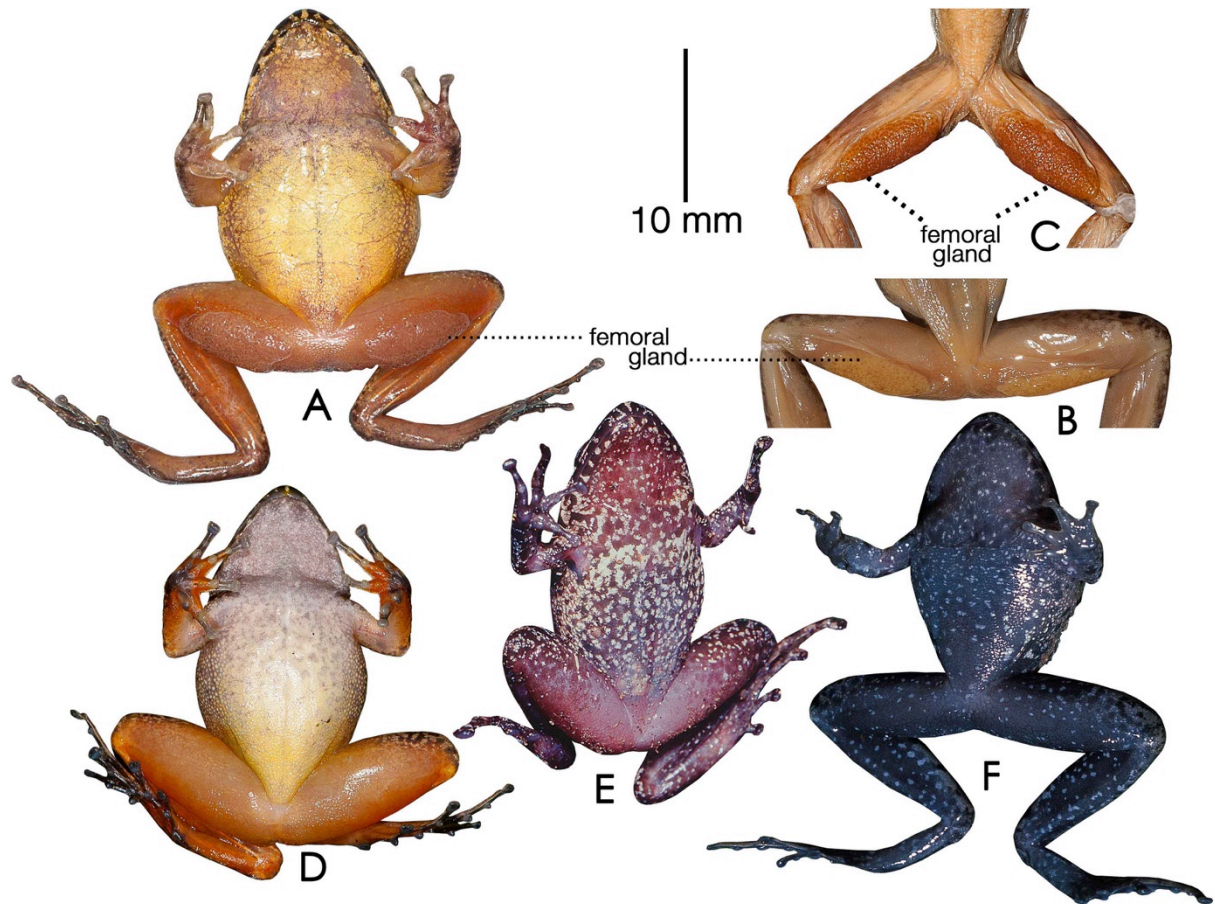
S1 Fig. Ventral coloration and femoral glands in ranixalid species. (A, B) Indirana semipalmata , male (SDBDU 2015.3034) with femoral glands. (A) In life. (B) In preservation. (C) I. gundia , male (MNHN 1985.0633) with femoral glands (in preservation). (D) I. brachytarsus , male (SDBDU 2015.2931), without femoral glands (in life). (E) Sallywalkerana leptodactyla , male (SDBDU 2003.40336), without femoral glands (in life). (F) S. phrynoderma , female (SDBDU 2002.1 181), having a distinct bluish-black ventral surface with scattered grey color speckles (in life).
