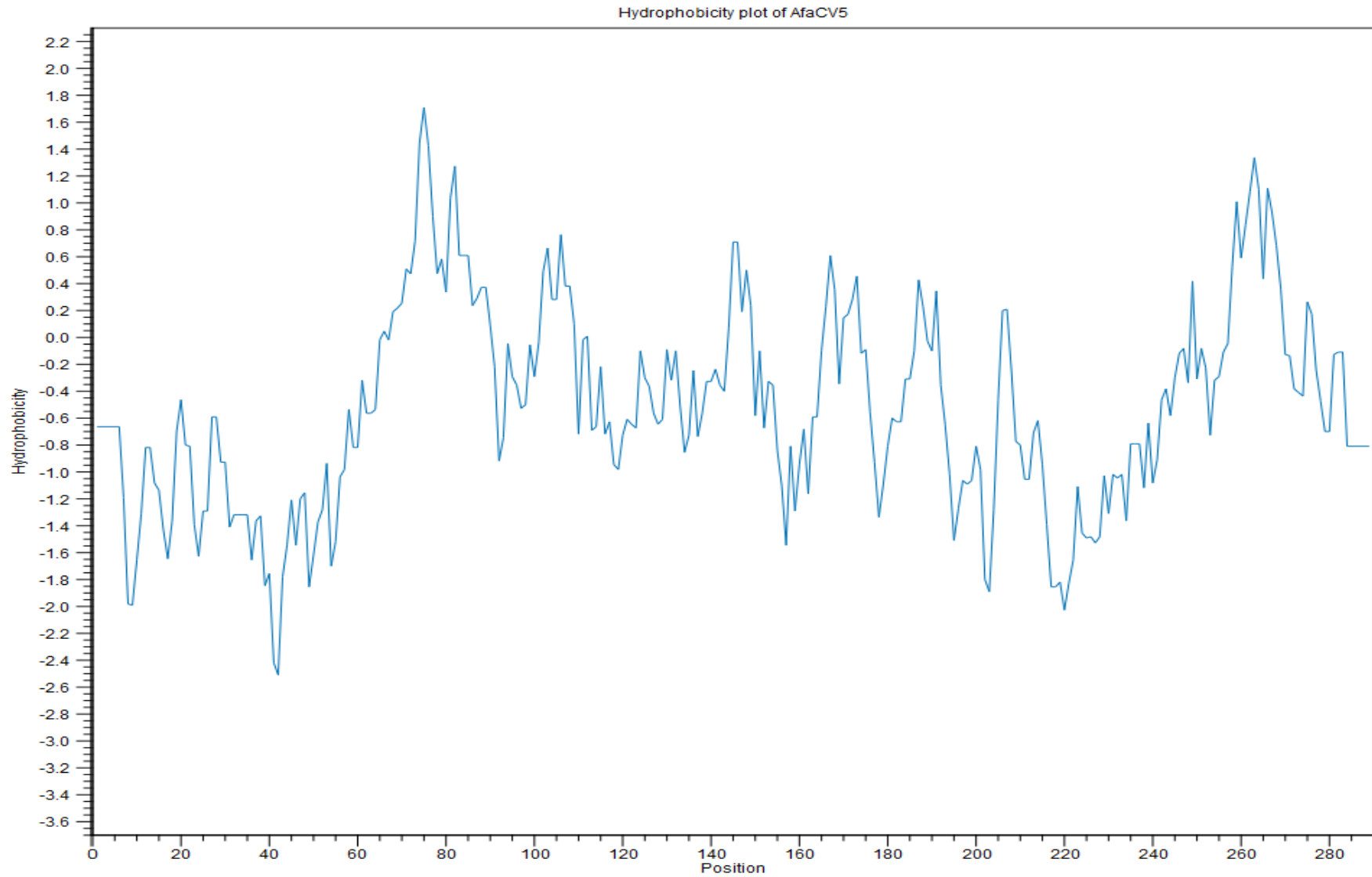
S4 Fig. Hydrophobic plot of hypothetical capsid protein of AfaCV5.
