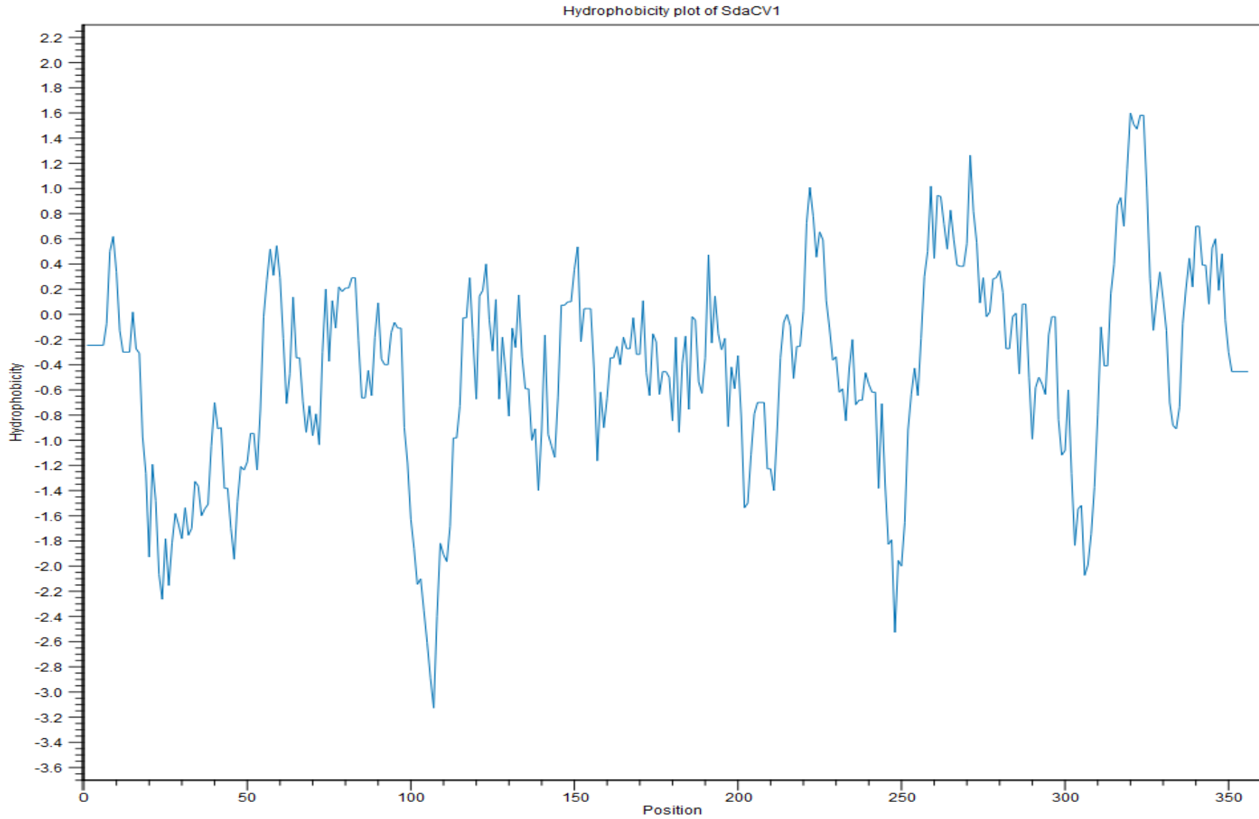
S5 Fig. Hydrophobic plot of hypothetical capsid protein of SdaCV1.
