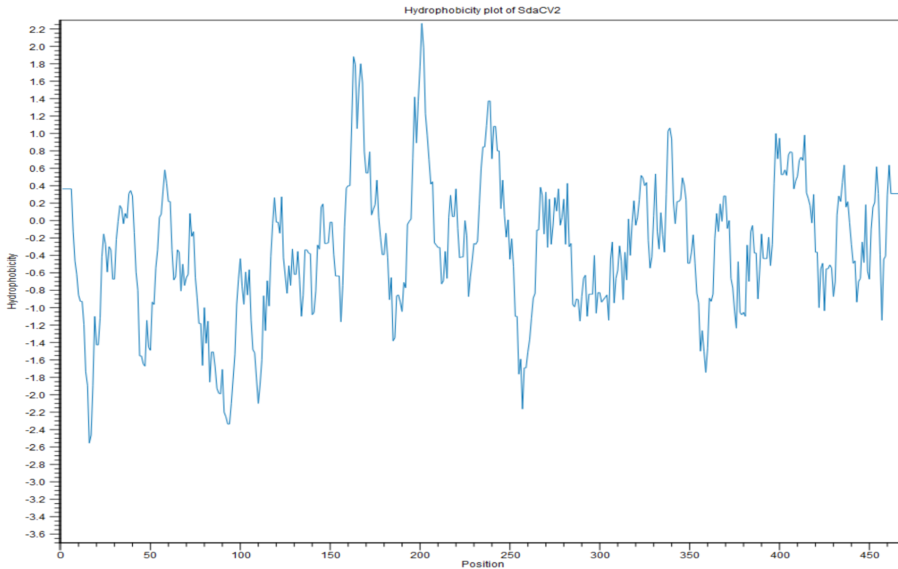
S6 Fig. Hydrophobic plot of hypothetical capsid protein of SdaCV2.
