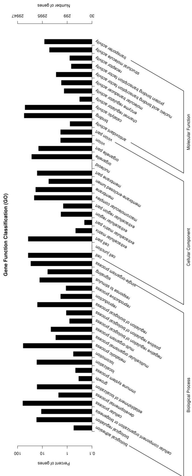
Figure S1 The information of gene function classification (GO) analysis
