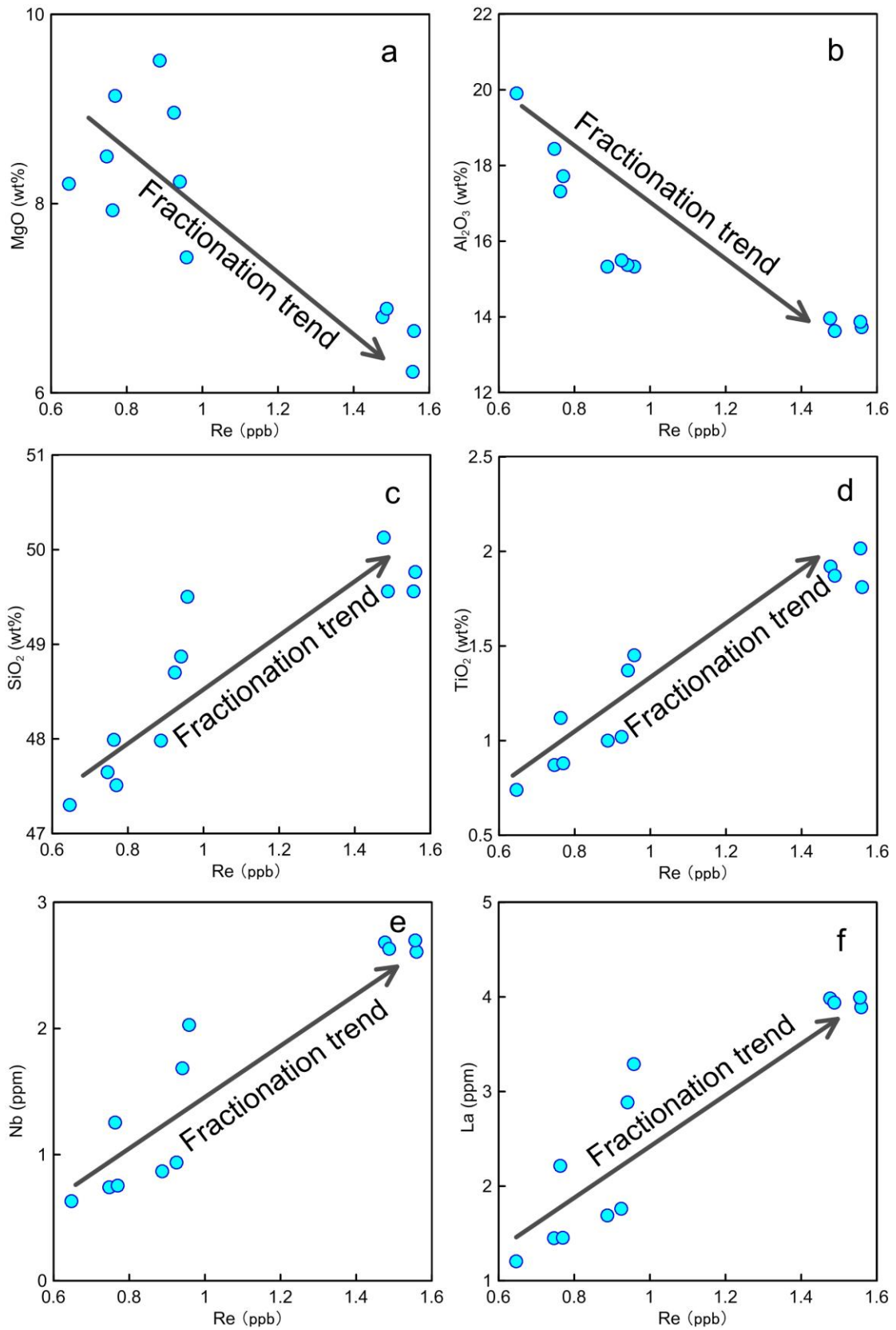
Figure S1 Plots showing relationships of Re with (a) MgO, (b) Al 2 O 3 , (c) SiO 2 , (d) TiO 2 , (e) Nb and (f) La.
