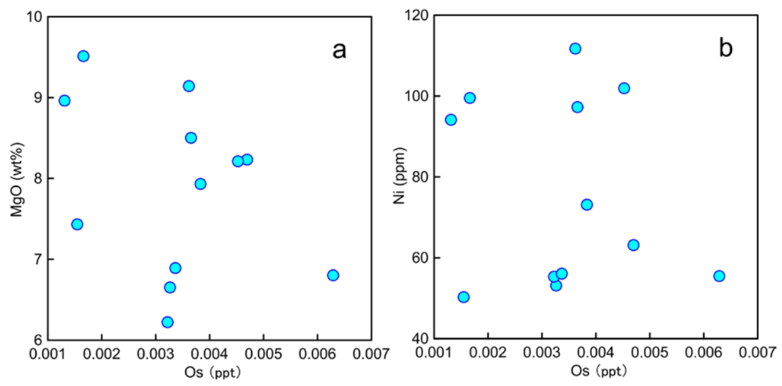
Figure S2. Plots showing relationships of Os vs. (a) MgO and (b) Ni.
