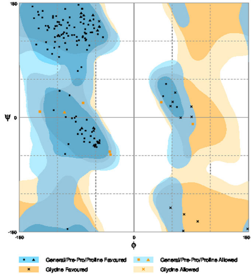
SUPPLEMENTARY FIG. S1. Ramachandran plot of Asp f1 modeled structure.
