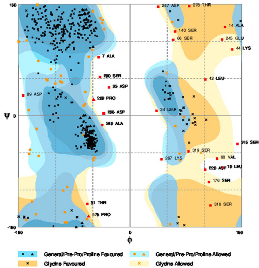
SUPPLEMENTARY FIG. S2. Ramachandran plot of Asp f5 modeled structure.
