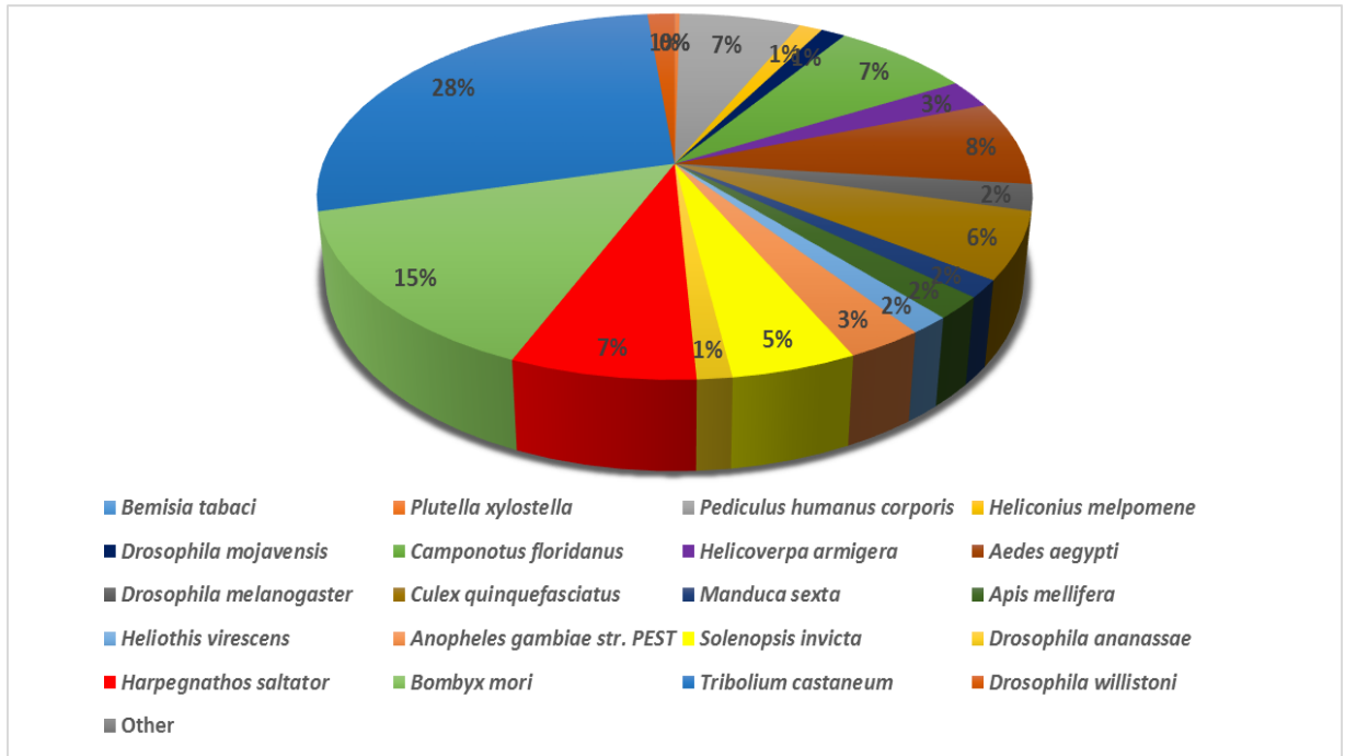
Fig. S1 Species distribution of the BLASTX results. This figure shows the species distribution of unigene BLASTX matches against the nr protein database (cutoff value e < 10^{-5} ).
