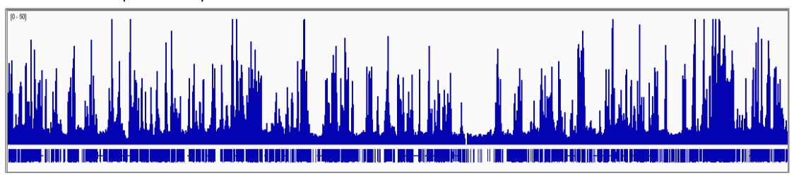
H2Av ChIP-Seq with Drosophila chromatin
