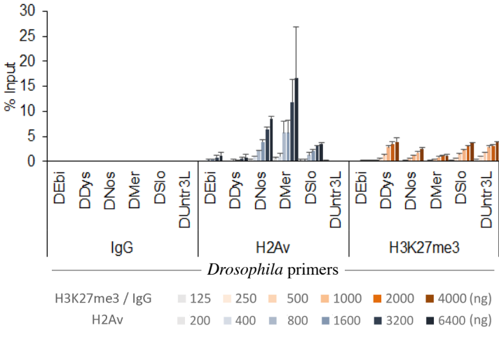
H2Av and H3K27me3 ChIP-qPCR with Drosophila chromatin
