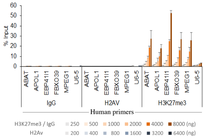
H2Av and H3K27me3 ChIP-qPCR with human chromatin
