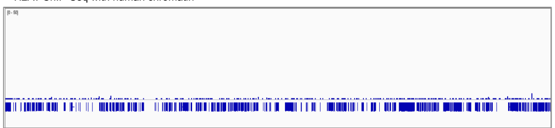
H2Av ChIP-Seq with human chromatin
