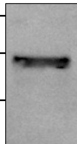
Figure S2. TrxIA-2 ic identification by western blot in eluted fractions from size exclusion chromatography and dithiothreitol reduction analysis.
