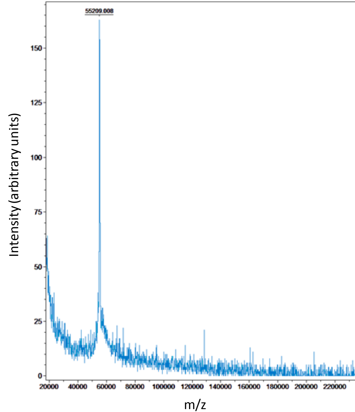
Figure S3. Mass spectrometric analysis of TrxIA-2 ic .
