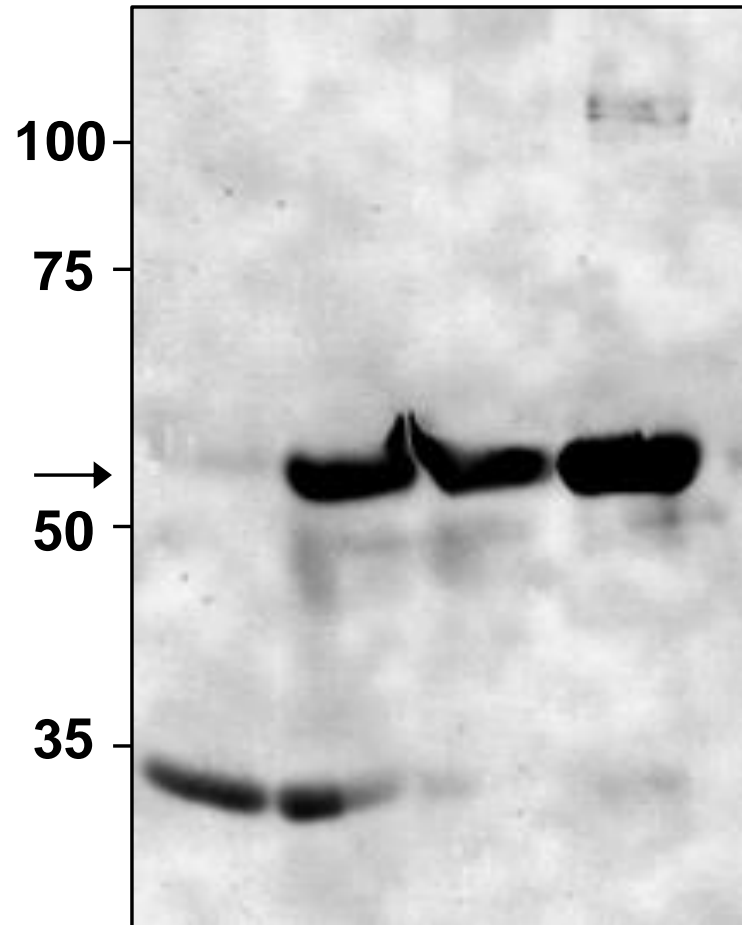
Figure S5. IA-2 ic expression as a fusion protein with Trx in E. coli GI724 inclusion bodies.
