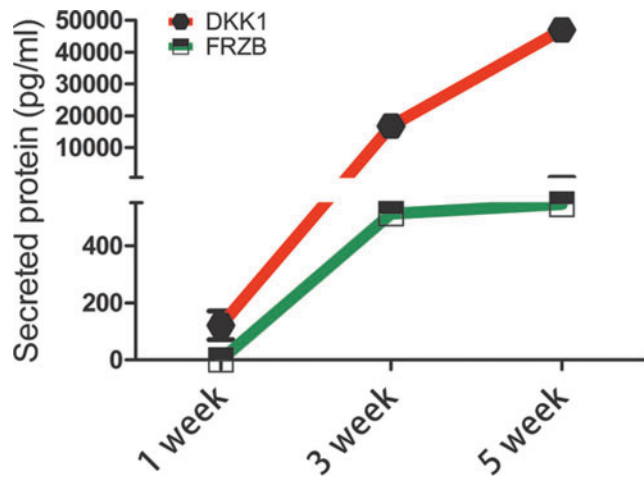
SUPPLEMENTARY FIG. S5. The protein expression of DKK1 and FRZB during chondrogenesis of hMSCs. hMSCs were cultured in chondrogenic differentiation medium containing dexamethasone and TGF- \beta . Culture medium was collected at indicated time point. DKK1 and FRZB protein levels were analyzed using ELISA.
