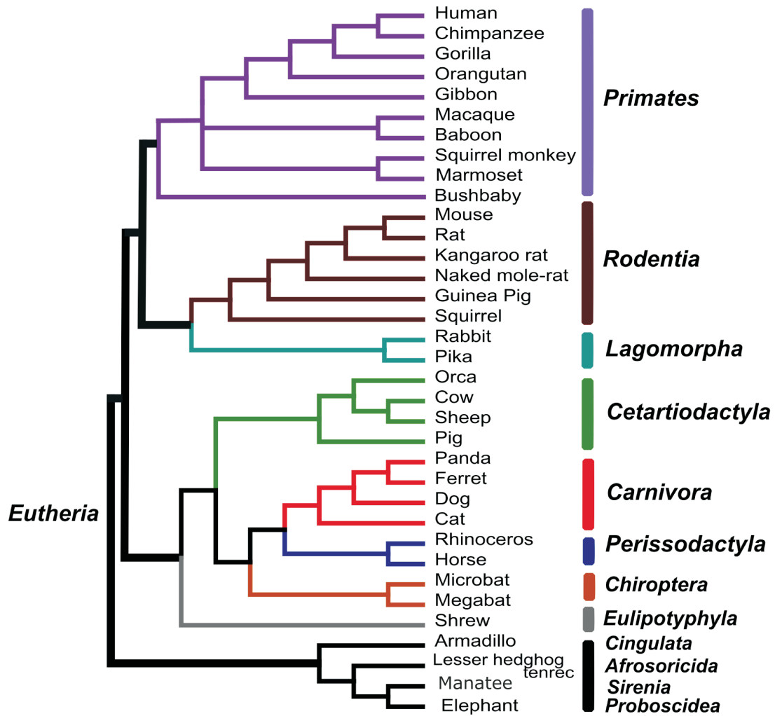
Figure S1 - Phylogenetic tree topology used in the analysis of molecular evolution. The analysis included 35 placental mammalian species (as described in the Materials and Methods section).
