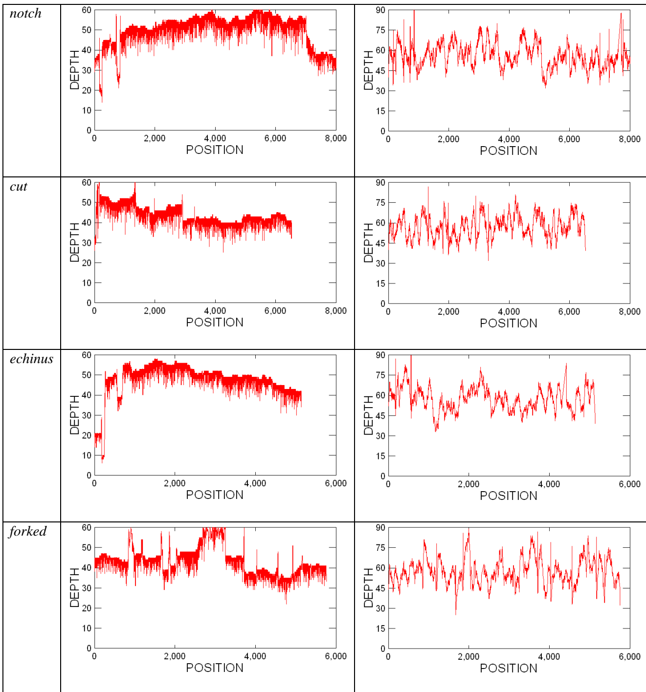
Supplemental Figure S12. Sequencing coverage for single copy Y-linked and X-linked genes. Left: PacBio reads. Right: Illumina reads. Reads were aligned with bwa to the coding sequence (CDS) of Y-linked (blue) or X-linked (red) Drosophila genes. Note that PacBio coverage is very low or zero in several regions of Y-linked genes, which never occurs with X-linked genes. Note also that Illumina coverage is fairly constant across all genes (except for exon duplications in the PPr-Y gene, and possibly in a few other Y-linked genes). The expected coverage is \sim 45x for both X-linked and Y-linked genes (reads came from males).
