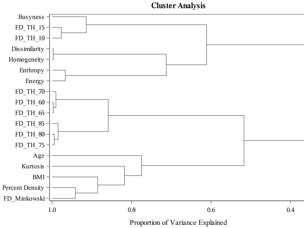
Figure S1. Dendrogram of cluster analysis of the top 15 features with PD, age and BMI. Similar features cluster together. Percent Density groups closely with BMI and age. The figure is restricted to the cases.
