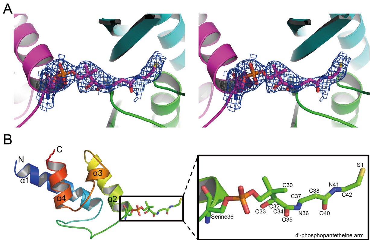
Supplementary information, Figure S5 The structure of holo-ACP in FabZ-ACP complex. (A) Stereo view of the omit electron density map contoured at 0.8 \sigma of the 4'-phosphopantetheine arm in FabZ-ACP complex. (B) The schematic diagram of holo-ACP. The atoms on the 4'-phosphopantetheine arm involved in the interactions are shown and labeled.
