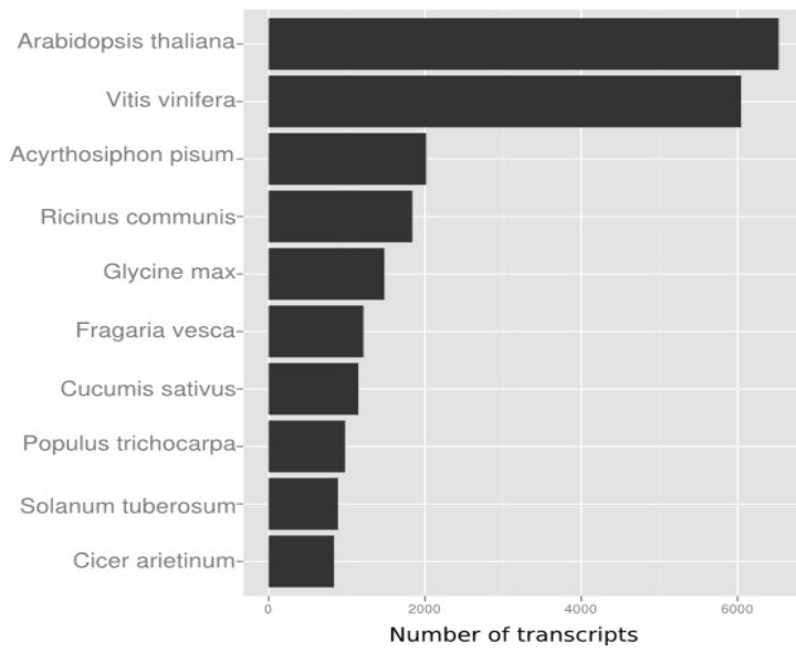
Figure S6. Plant species with the most protein sequence similarity to P. lambertiana transcripts
