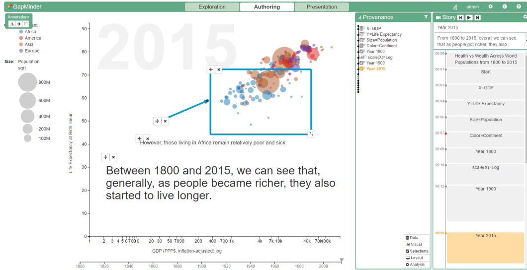
Figure S1: Screenshot of the Gapminder-inspired application showing the same state as the usage scenario in authoring mode. Vistory: http://vistories.org/v/gapminderA .
