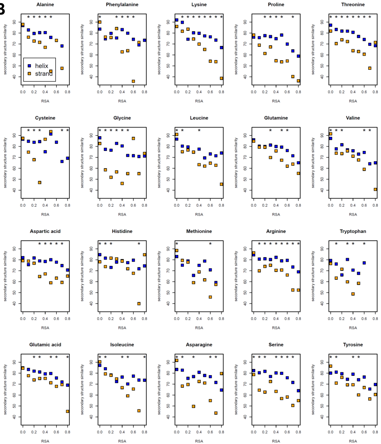
S5 Figure – continued. B) \alpha/\beta domains.
