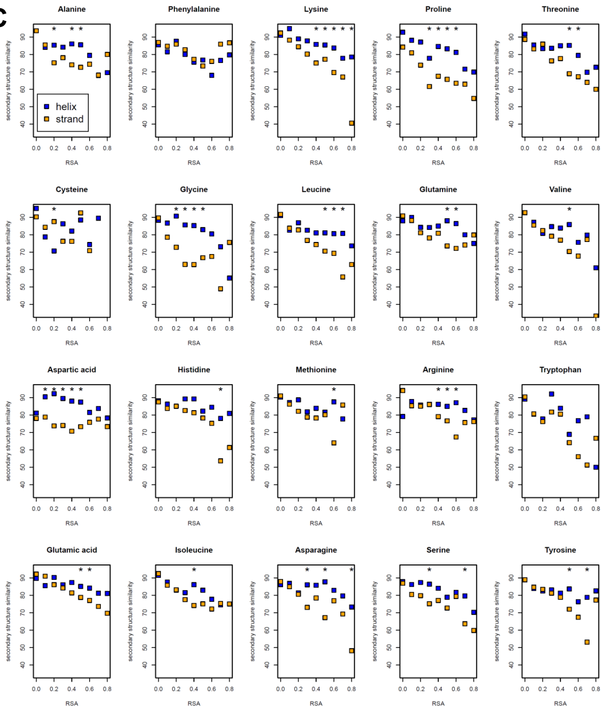
S5 Figure - continued. C) \alpha+\beta domains.
