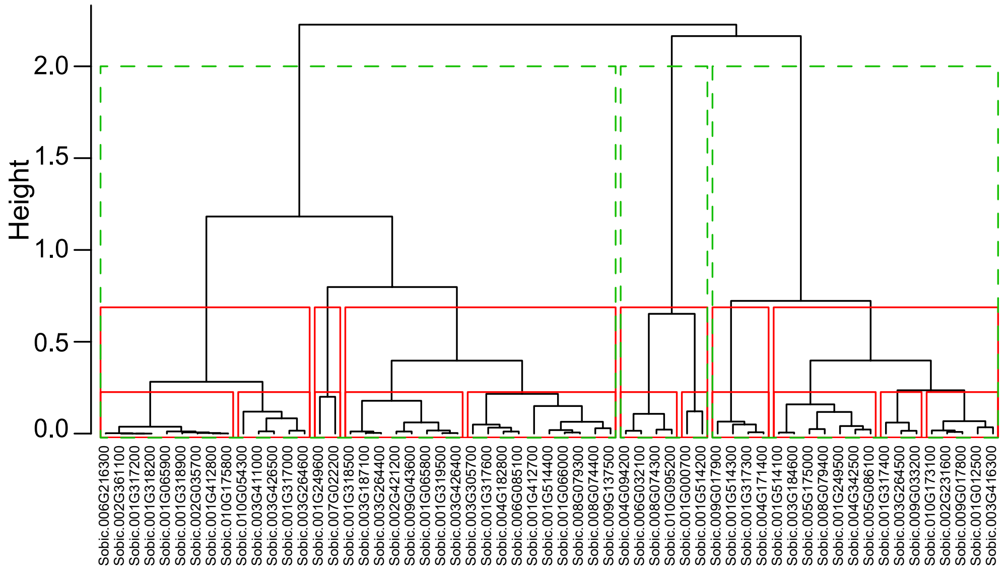
Additional file 5. Plot of the dendrogram from the hierarchical clustering of expressed GST genes, showing the relation between the 6 clusters and the 12 subgroups marked by red boxes in the bottom of the figure. The gene names belonging to the different clusters are listed below. The 6 clusters can be divided into 3 clades (marked by green dashed lines) containing genes with an overall similar profile.
