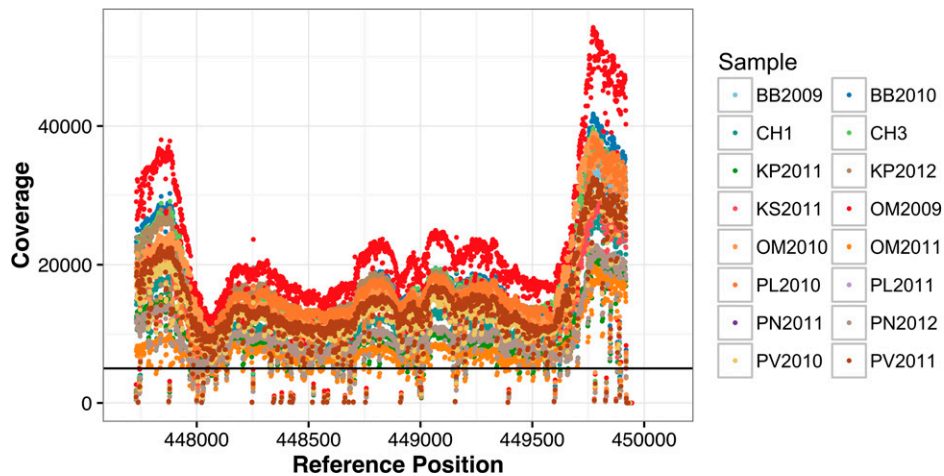
SUPPLEMENTAL FIGURE 2. Distribution of coverage by nucleotide position of bases with high quality ( q > 20 ) for each of the pooled samples. The black line represents base coverage below or above 5,000-fold coverage.
