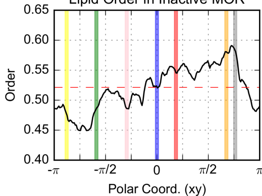
Lipid Order in Inactive MOR
