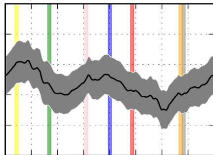
Bilayer Thickness in Active MOR
