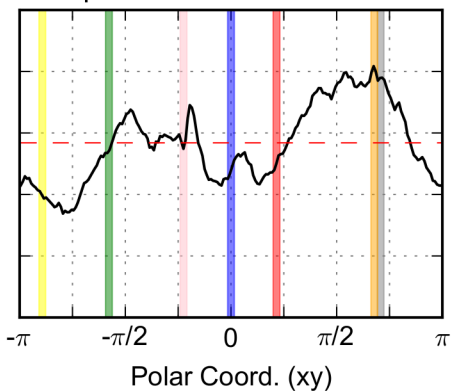
Lipid Order in Active MOR
