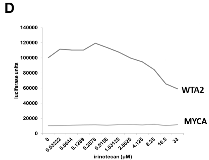
Suppl. Fig. 4. Luciferase reporter assays of four candidate HMGA2 antagonists in 96 well-formats.
