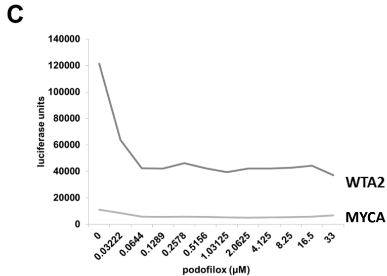
Suppl. Fig. 4. Luciferase reporter assays of four candidate HMGA2 antagonists in 96 well-formats.
