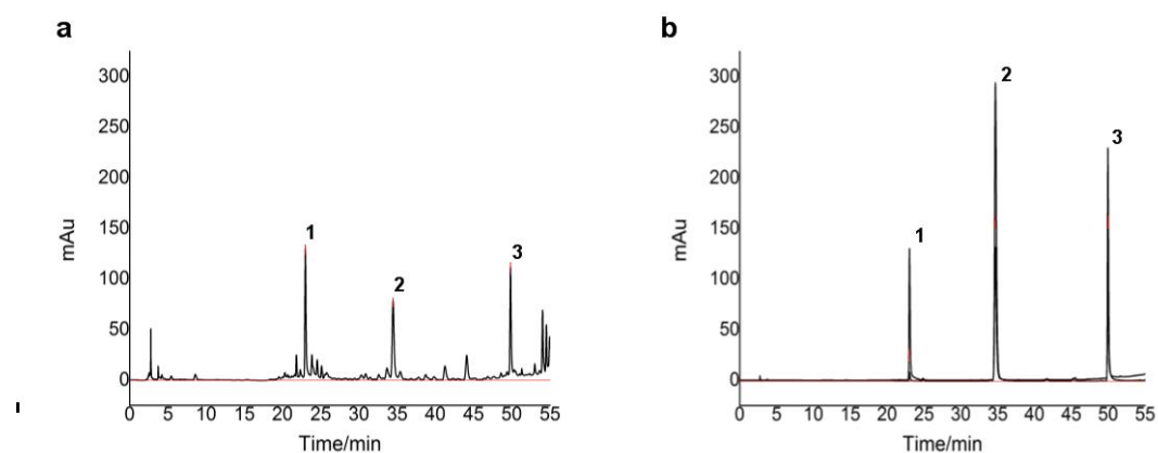
Supplementary Figure 1. HPLC chromatogram of main active components in an aqueous extraction of HQT. (a) aqueous extract of HQT. (b) Standards: 1, paeoniflorin; 2, baicalin; 3, baicalein.
