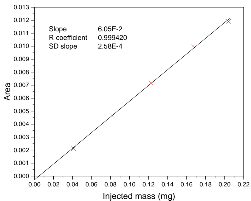
Figure S2. RI peak area plotted vs. the injected mass for five different concentrations of Rhamnogalacturonan-I. The dn/dc can be obtained from the slope, which depends on the RI detector constant and the dn/dc .
