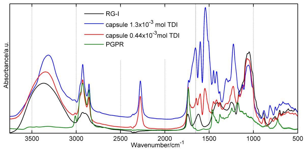
Figure S3. FTIR data including the surfactant PGPR.
