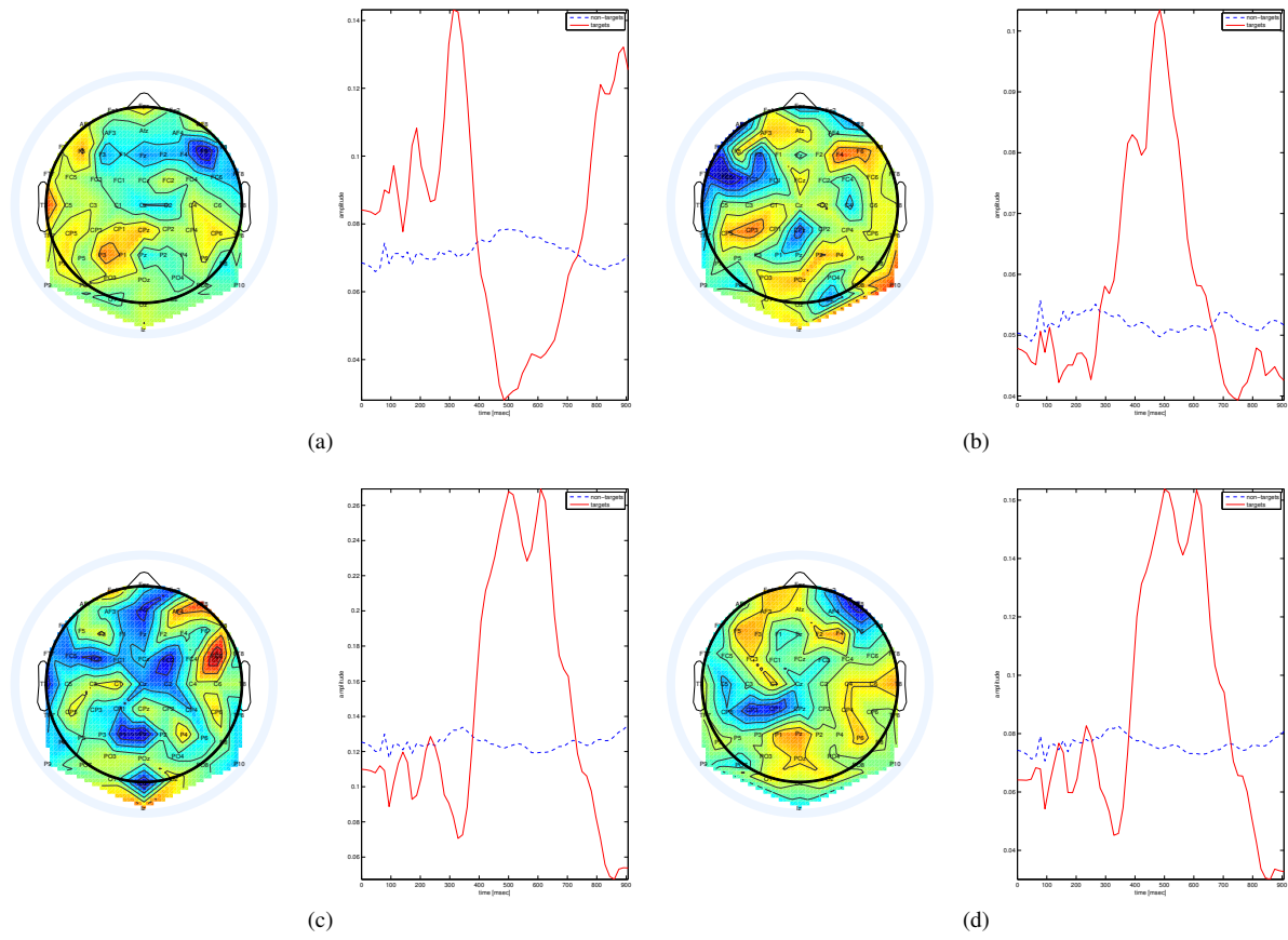
Figure S4. Weights of the first convolutional layer in the EEG network from several subjects/sessions, where we can see the variability across the data.
