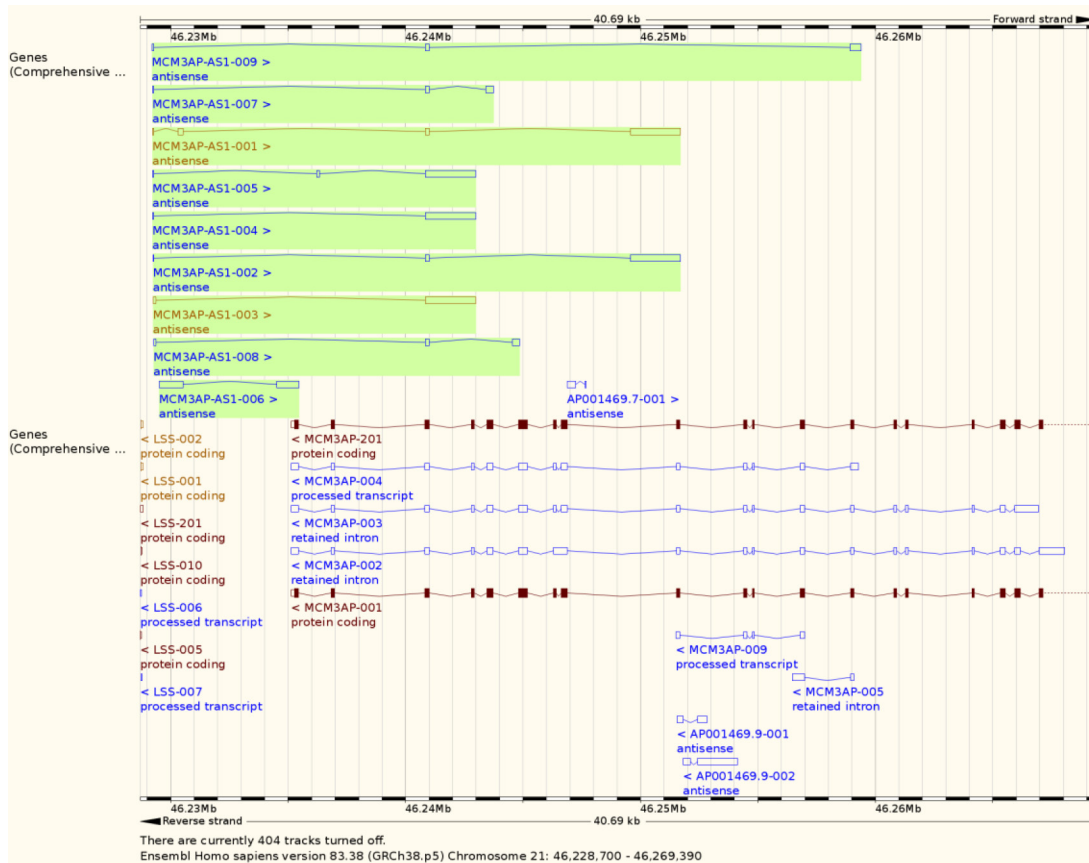
Supplementary Figure S1: Genomic location of MCM3AP and MCM3AP-AS according to Ensembl Genome Browser.
