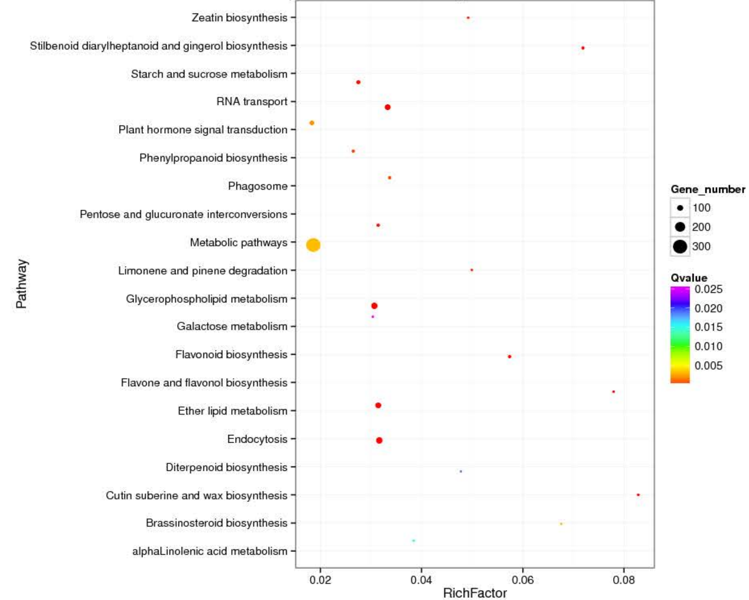
Top 20 Statistics of Pathway Enrichment for CK14-vs-T14
