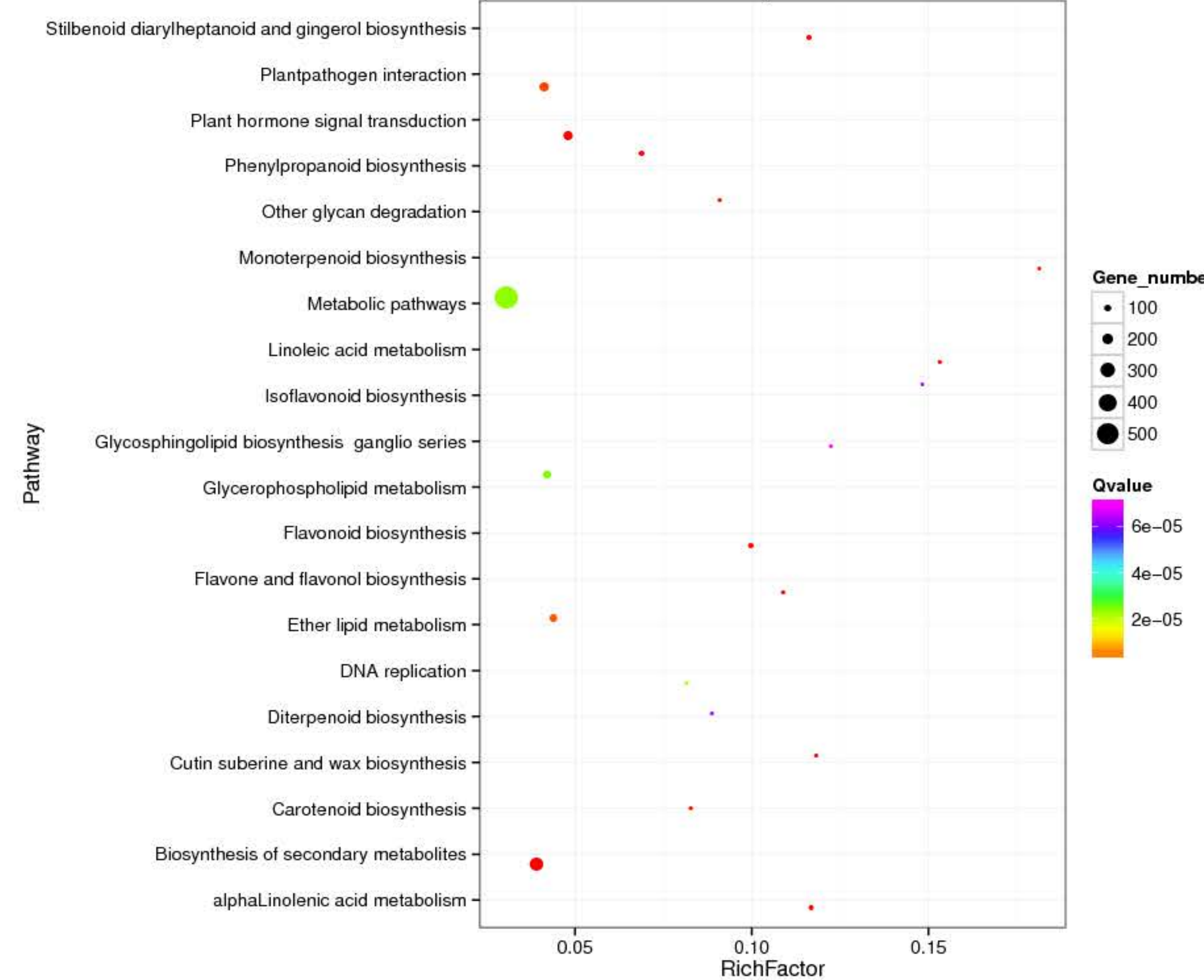
Top 20 Statistics of Pathway Enrichment for CK7-vs-T7
