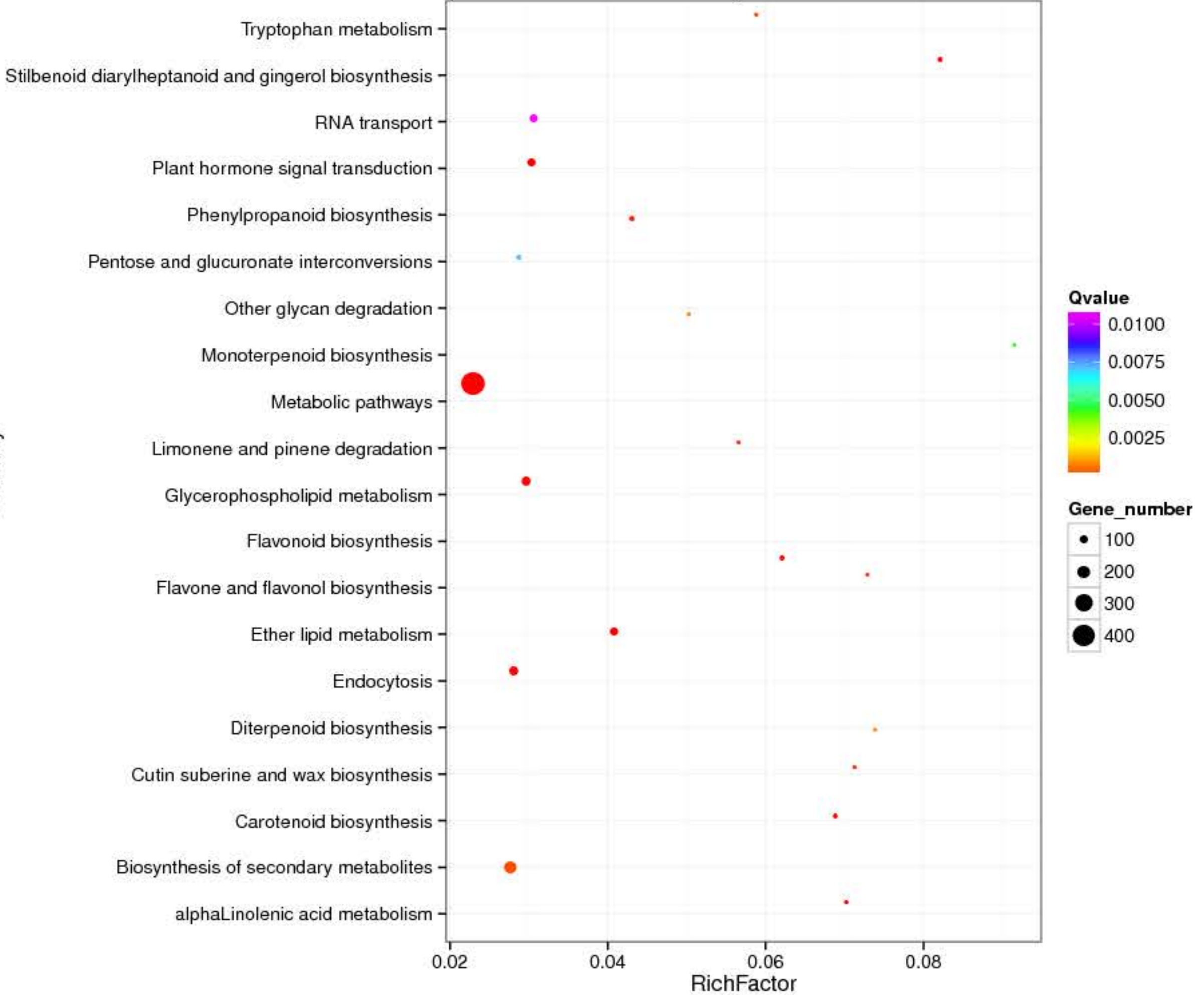
Top 20 Statistics of Pathway Enrichment for CK3-vs-T3
