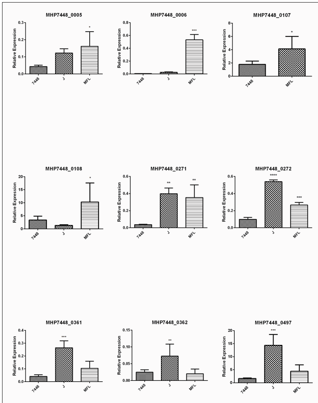
Supplementary Figure S2: Experimental validation through qPCR assay of palindrome elements comparison in adhesin coding genes.
