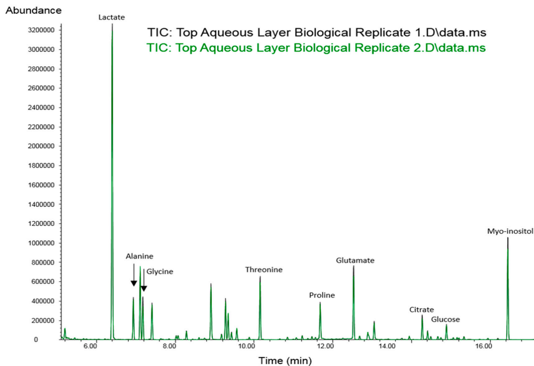
Figure S1. Total ion chromatogram (TIC) of the top aqueous layer generated using the described biphasic extraction procedure. Two biological replicates from C2C12 myoblasts were analysed via GC-MS using the MOX-TMS derivatizing strategy, confirming the presence of polar intracellular metabolites.
