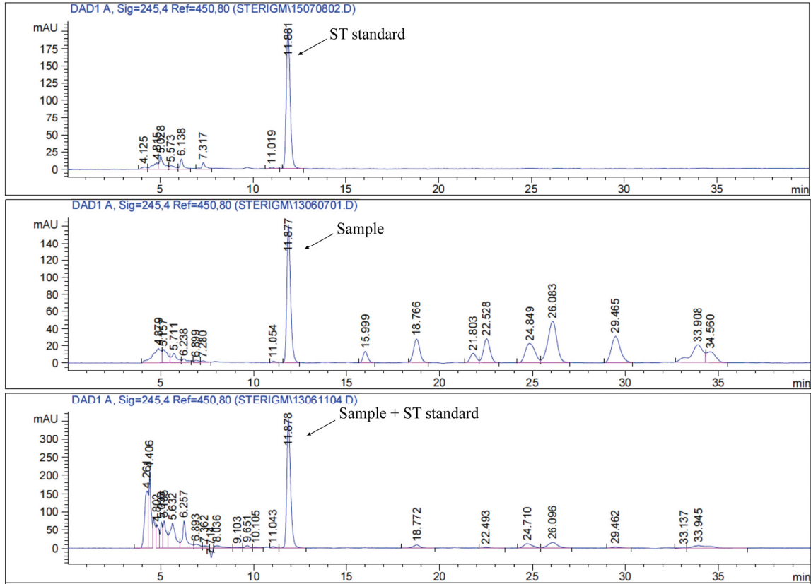
Figure S2. RP-HPLC-UV chromatograms showing an ST standard, a sample and a standard addition procedure.
