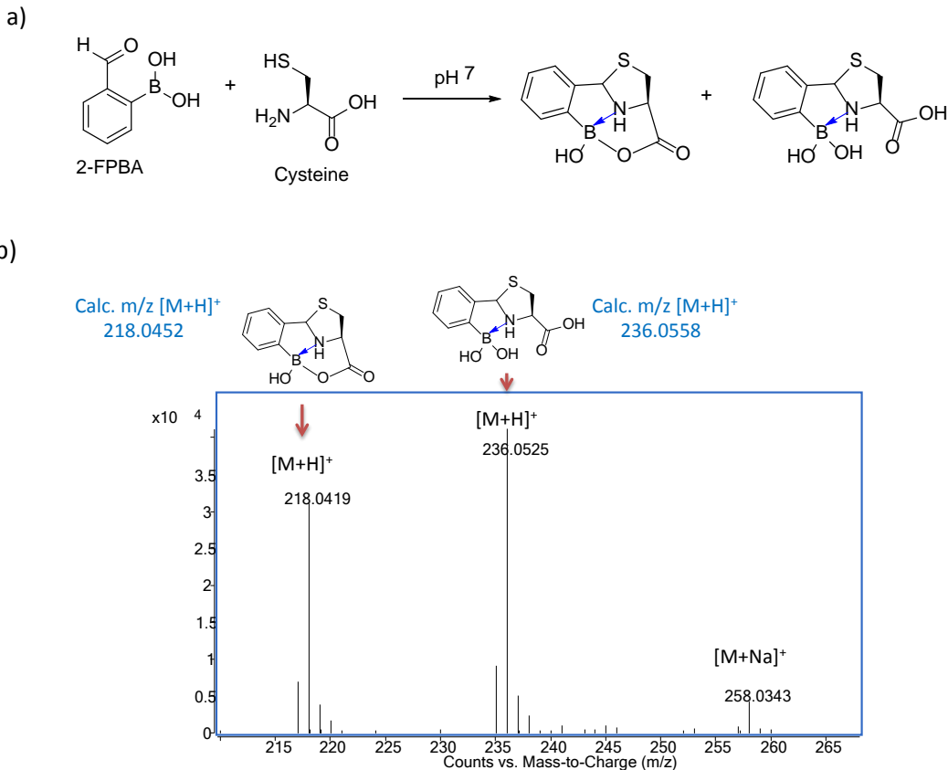
Figure S3. a) Illustration and b) mass-spec proof of the two species generated by conjugation of 2-FPBA with L-cysteine.
