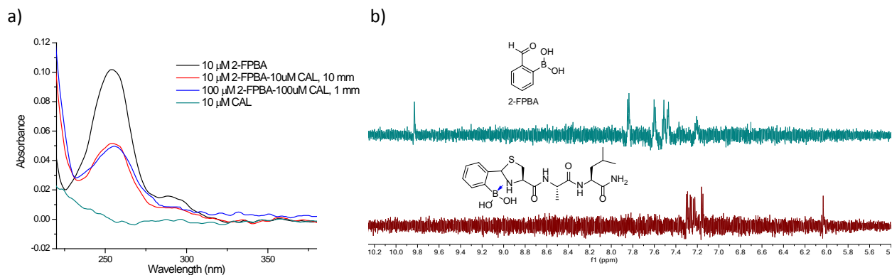
Figure S5. a) UV-vis profile overlay of 2-FPBA-CAL complex at 10 and 100 \mu M to confirm the complete conjugation at 10 \mu M. b) ^1\text{H-NMR} data (600 MHz at 25 ^\circ\text{C} with 160 scans) showing complete conjugation of 2-FPBA and CAL at 100 \mu M.
