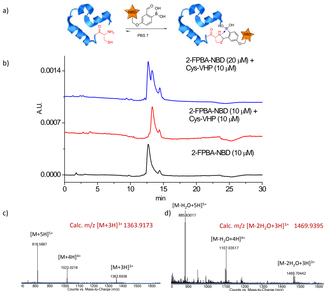
Figure S6. a) Scheme for N-terminal protein labeling through TzB complex formation. b) HPLC traces (Method III) for 2-FPBA-NBD alone and its mixtures with Cys-VHP. A small impurity ( \sim 6\% ) at 14.4 min appeared due to the oxidation of boronic acid to phenol, which was confirmed by mass spectrum analysis. c) Mass spec data of Cys-VHP before and d) after conjugation with 2-FPBA-NBD. Water loss is commonly seen in the mass-spec results of boronic acid-presenting compounds. 1
