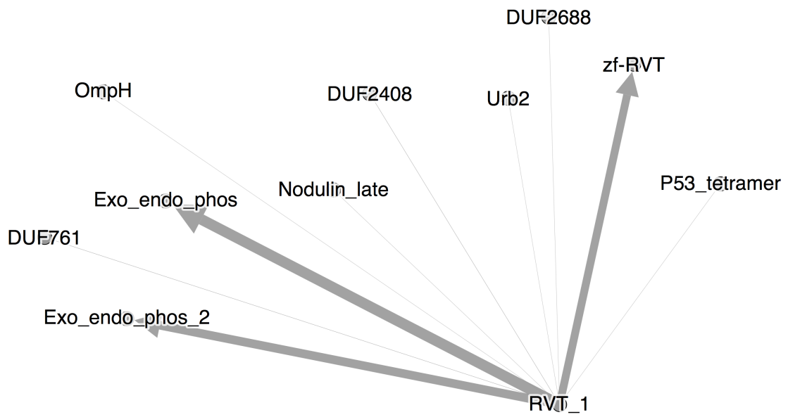
Figure 6c: Amphibia ORF2p domains
