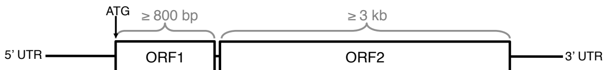
Figure 4: Intact ORFs: An ORF is considered intact if it is at least 80% of the expected length, with a start codon, stop codon, and no debilitating mutations in between (e.g. premature stop codons, large stretches of ambiguous nucleotides). ORF1 has the additional requirement of starting with a methionine start codon (ATG). L1 sequences were extended by 1kb either side during identification of the ORFs, in case the ORF start/stop codons were outside of the extracted L1 sequence. ORF1 and ORF2 were also confirmed by alignment and tested for similarity to known domains, as described in the main text.
