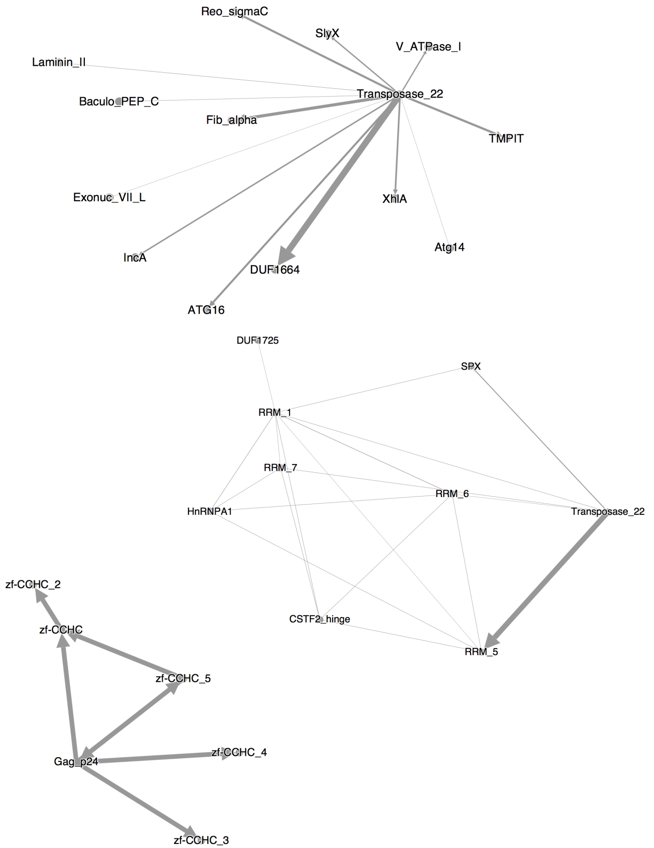
Figure 7a: Mammalia ORF1p domains
