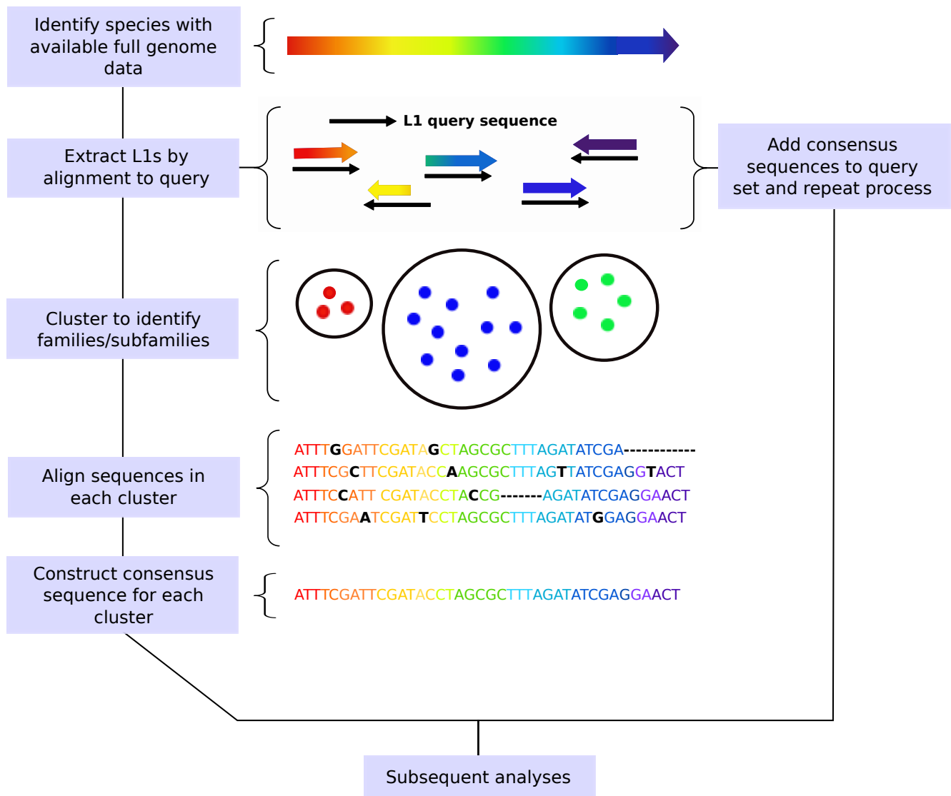
Figure 2: L1 extraction pipeline: Consists of an iterative query-driven method based on sequence similarity. Query L1 sequences from different species are concatenated into one file. This is used to extract similar sequences from each of the 503 genomes. For each species, the L1 hits are clustered and then aligned to generate a consensus sequence for each cluster (subfamily). These consensus sequences are then added to the query file and the process is repeated. This pipeline was initially repeated three times; then, the independent TBLASTN approach was used to generate species-specific queries; then, this pipeline was repeated a final two times: first with the species-specific queries and then with all individual L1s (more than 3 million sequences) .
