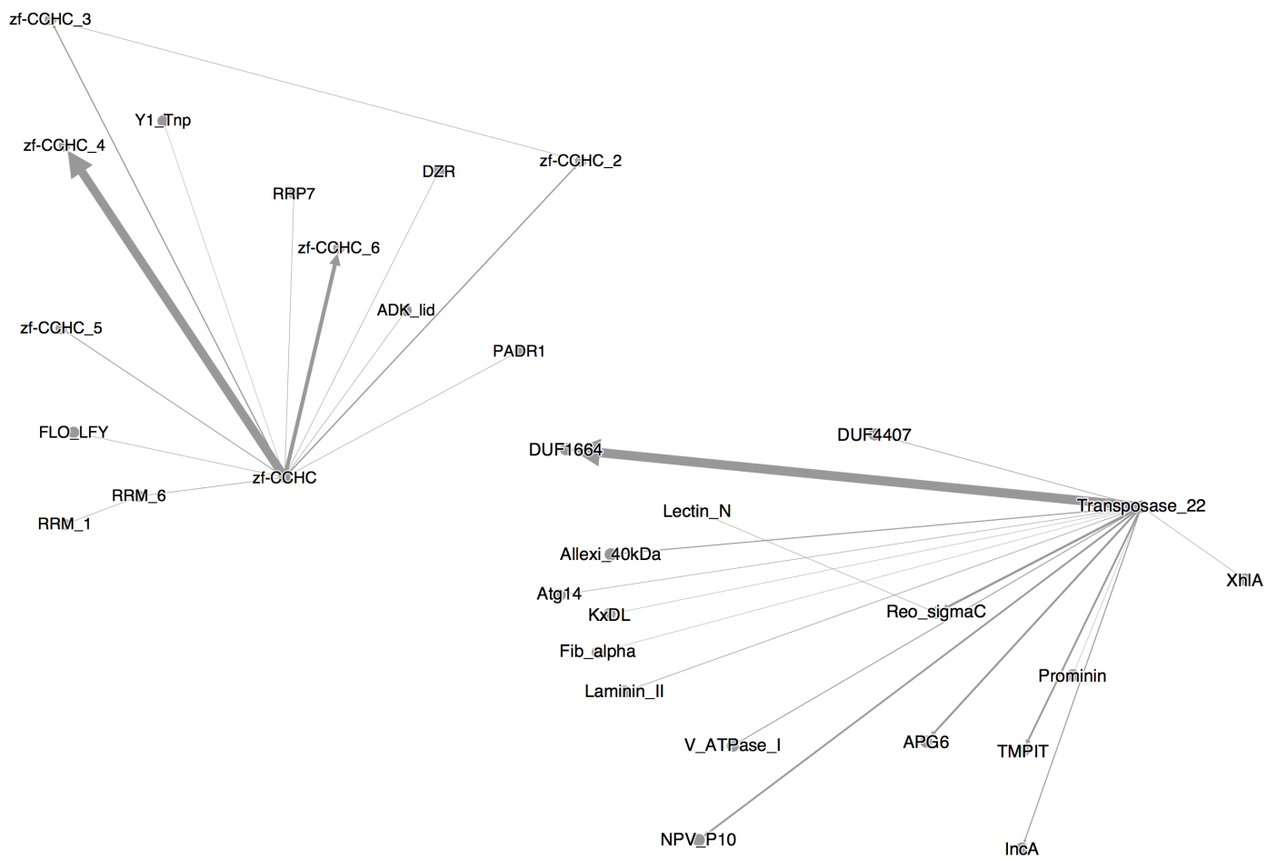
Figure 7b: Sauropsida ORF1p domains
