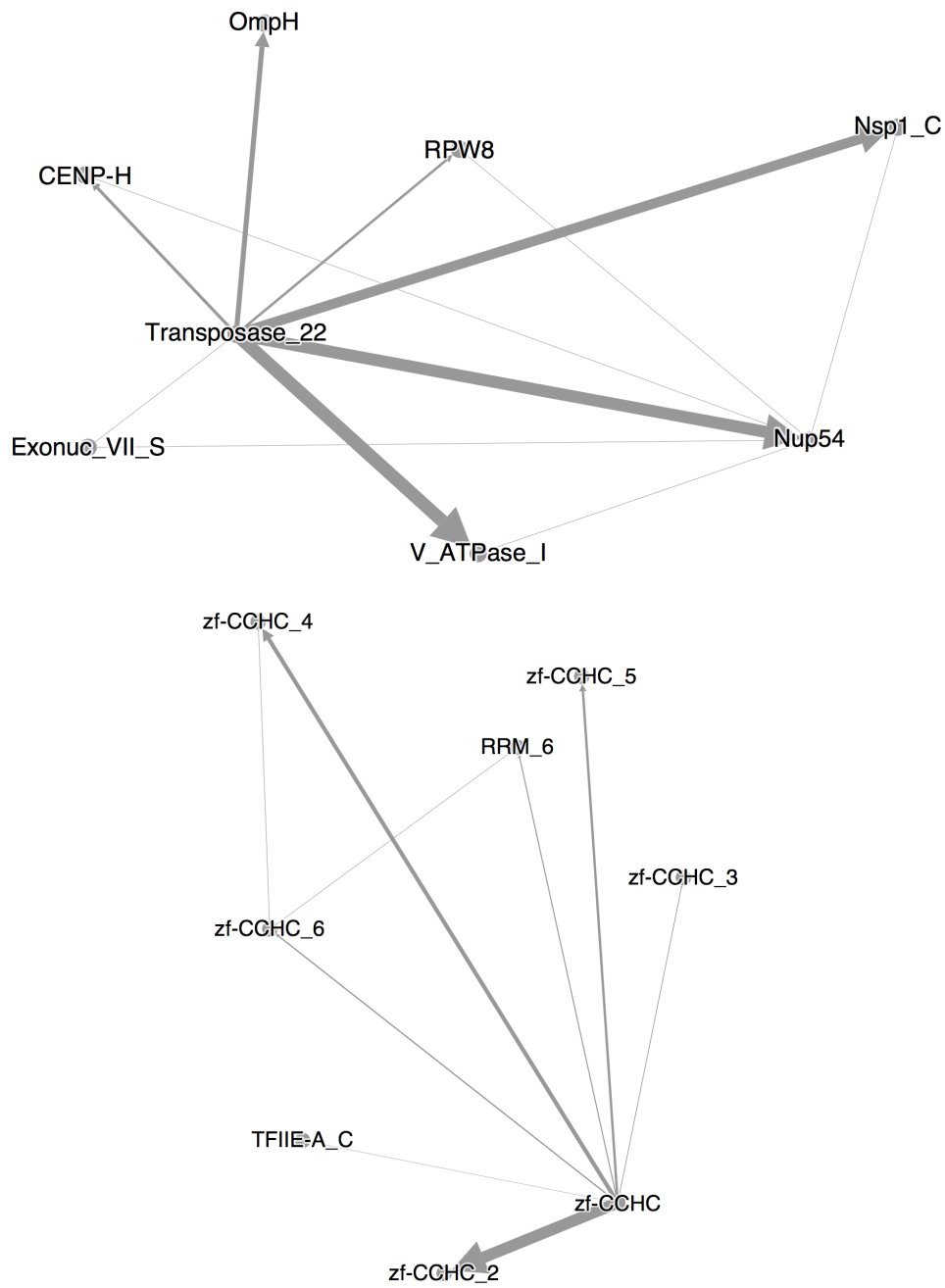
Figure 7d: Neopterygii ORF1p domains
