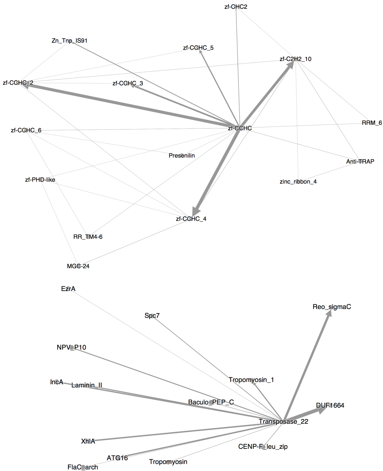
Figure 7f: Other, primitive non-mammalian species - ORF1p domains
