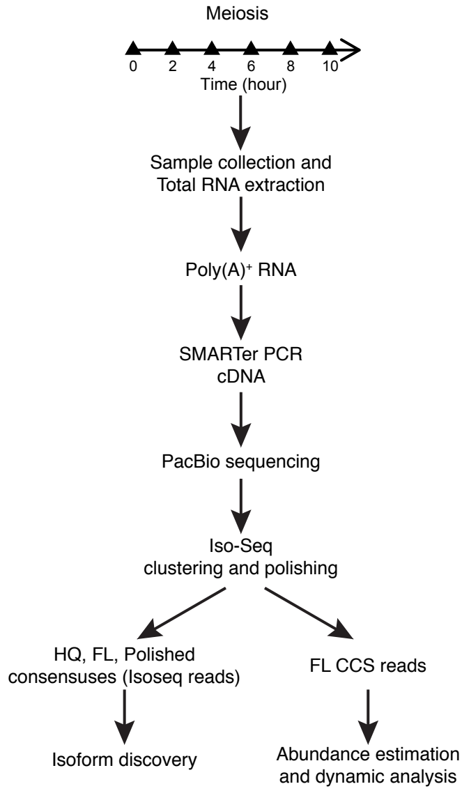
Supplemental Figure S1. A workflow to characterize the diversity and dynamics of transcriptomes in S. pombe meiosis.
