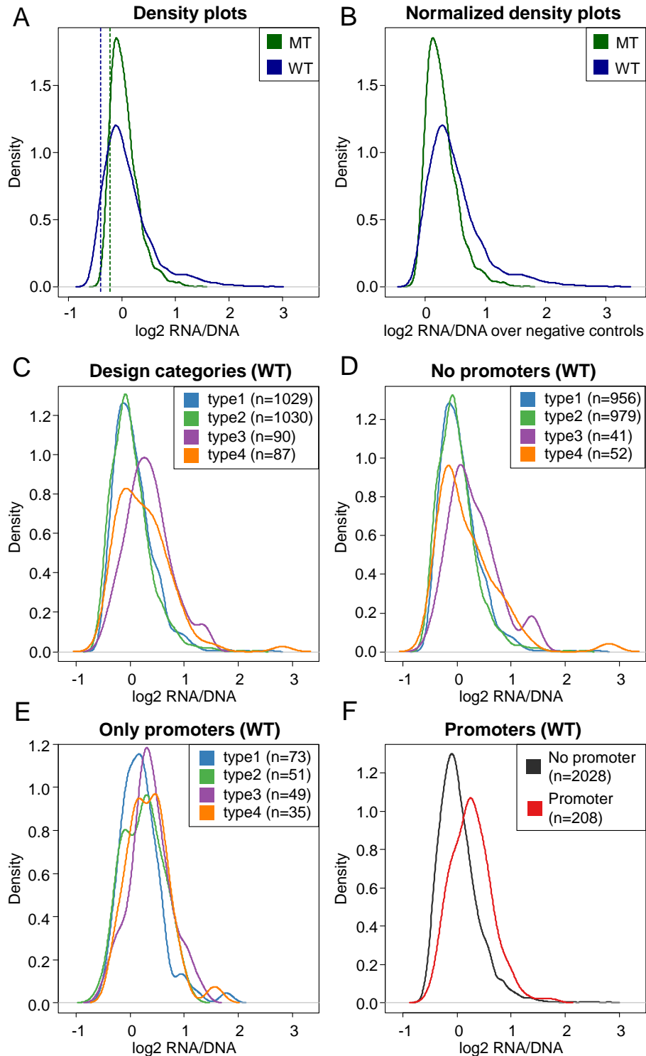
Supplemental Figure S16. Density plots of RNA/DNA ratios: (A) RNA/DNA ratios observed between the MT and WT experiments with dashed lines marking the average value of the two negative controls. (B) Overlay of the RNA/DNA ratios of MT and WT experiments after normalizing to the average of the two negative controls. (C-D) Density plots of the WT RNA/DNA ratios by design categories and separating promoter (defined as within 1kb of a TSS) and non-promoter sequences.
