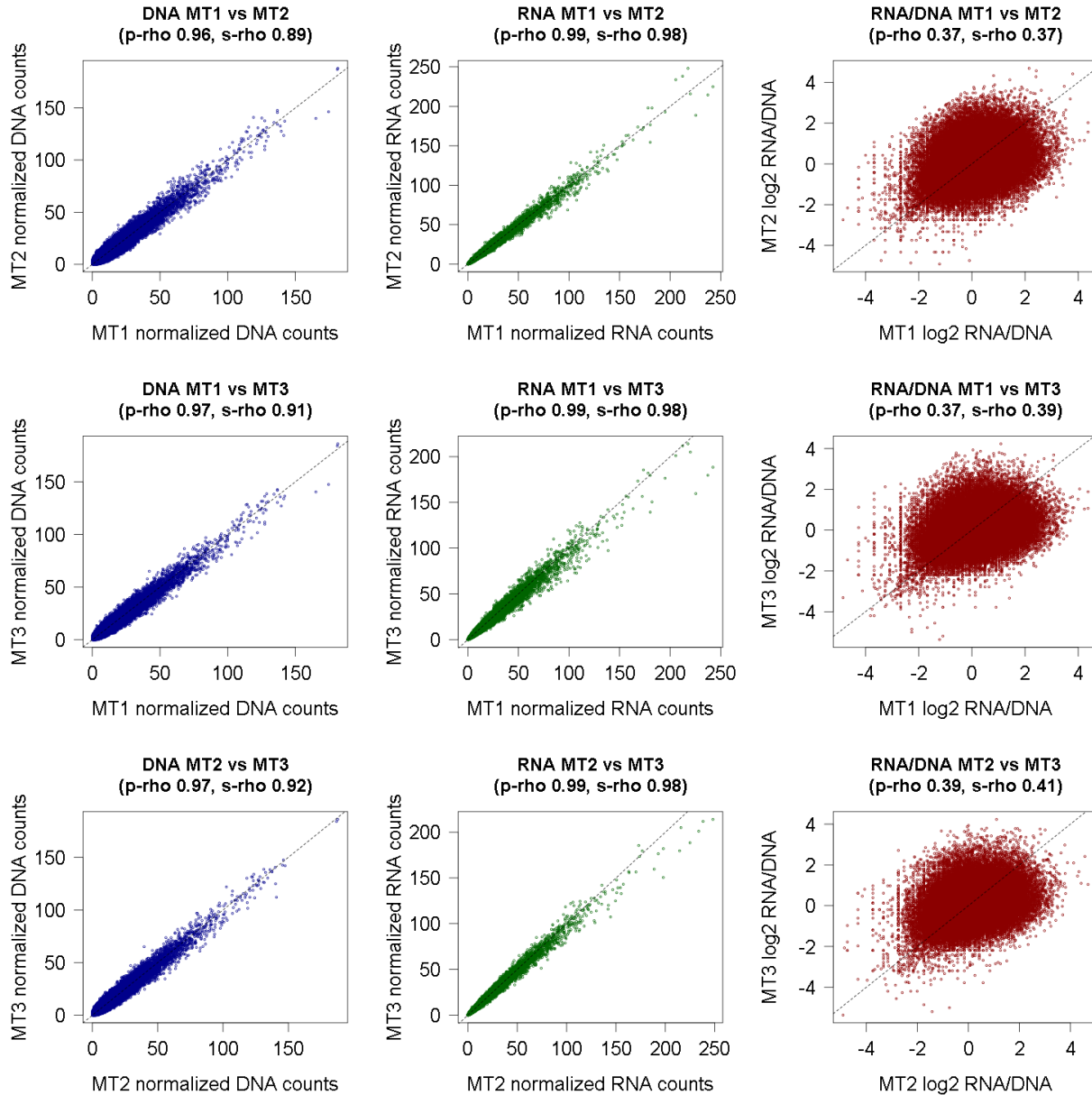
Supplemental Figure S6. Correlation (Pearson/p-rho and Spearman/s-rho) of DNA tag counts (left column), RNA tag counts (middle column) as well as RNA/DNA ratios (right column) for pairwise comparisons of three mutant-integrase (MT) library replicates (rows). These are for individual barcodes, i.e. before summing across barcodes representing the same candidate enhancer sequence.
