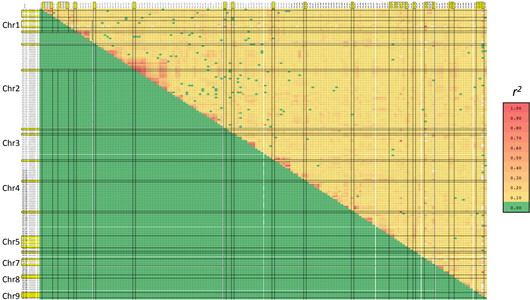
Figure S4 Pairwise |r^2| for 167 SNPs across L. sativa pseudo-chromosomes 1, 2, 3, 4, 5, 7, 8, 9 from assembly 'Lsat-1_v4'. Yellow highlighting indicates SNPs associated with Nasonovia count data. The SNPs surrounding the significant SNPs are included for regional reference to the surrounding LD.
