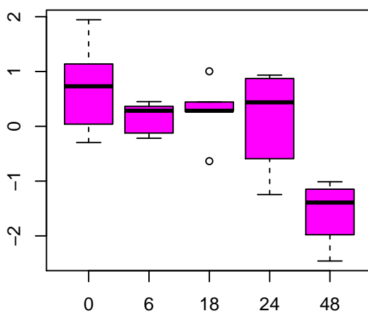
isoleucine
