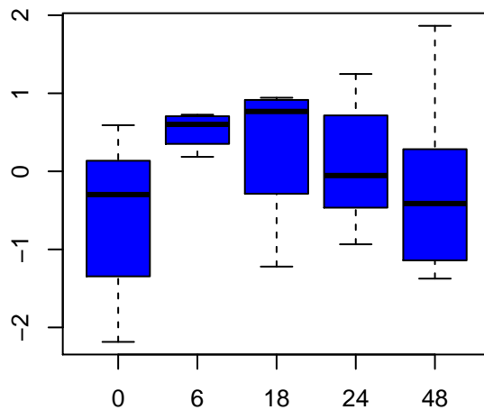
cis-vaccenate (18:1n7)
