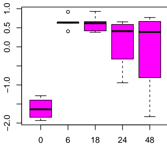
trans-4-hydroxyproline
