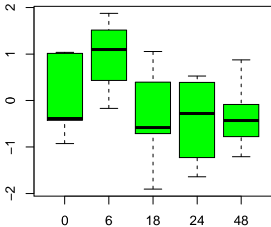
methionine sulfoxide
