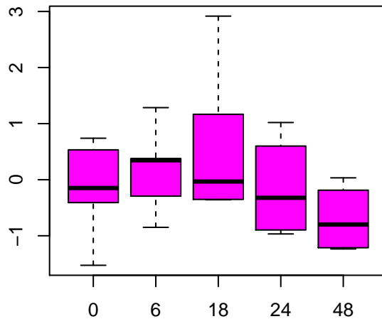
cis-vaccenate (18:1n7)
