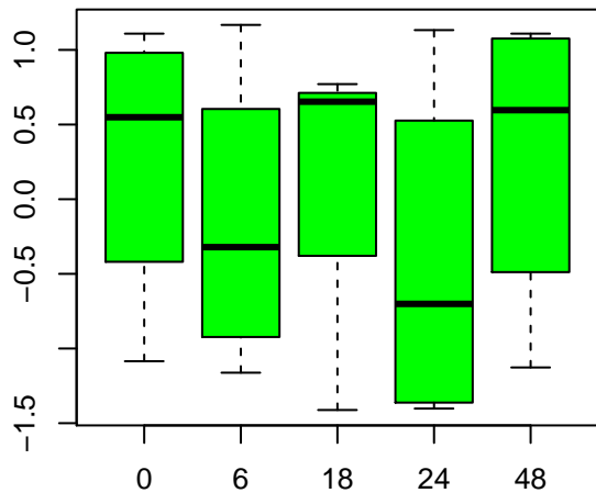
adenosine 5'diphosphoribose
