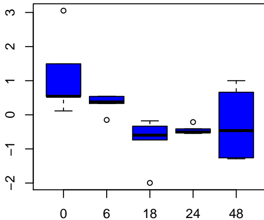
methionine sulfoxide
