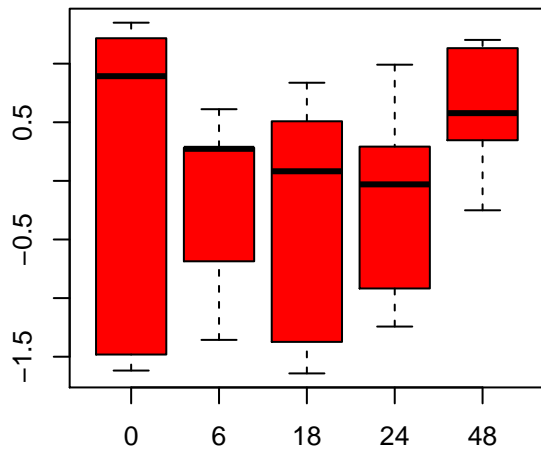
proline
