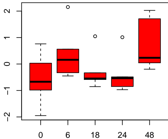
phenylalanine
