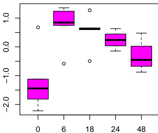
cholesterol
