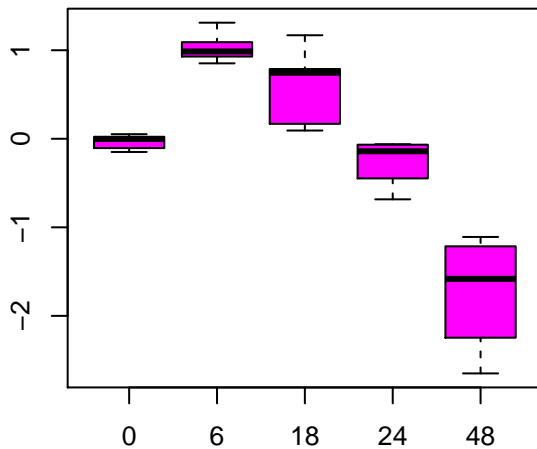
gamma-glutamylglutamate
