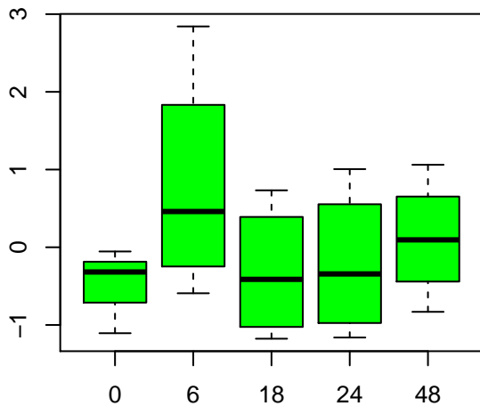
phenylalanylglycine
