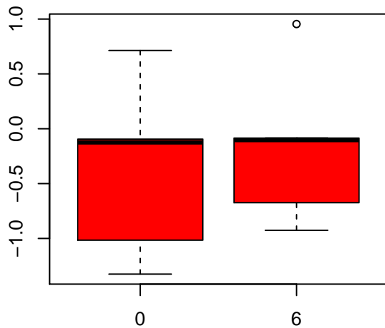
nicotinamide adenine dinucleotide (NAD + )
