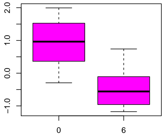
1-palmitoylplasmenylethanolamine*
