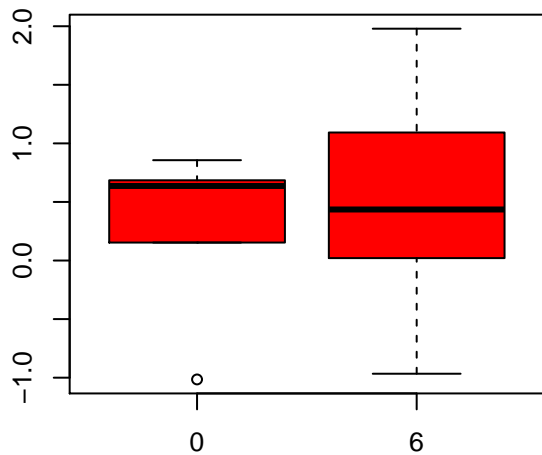
isoleucylalanine
