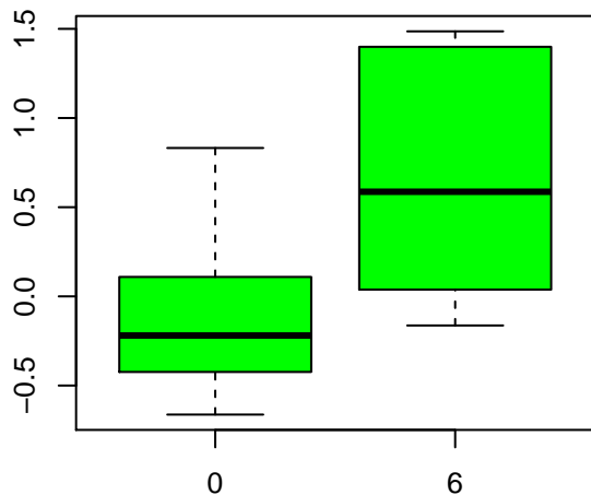
adenosine 5'-diphosphate (ADP)
