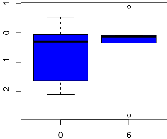
leucylalanine
