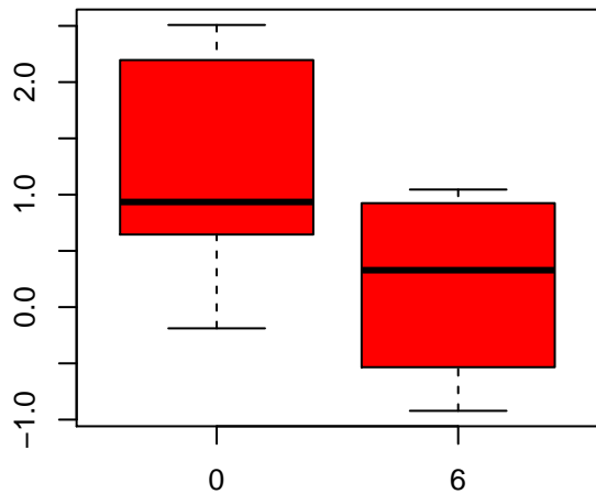
pro-hydroxy-pro
