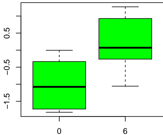
cytidine 5'-diphosphocholine
