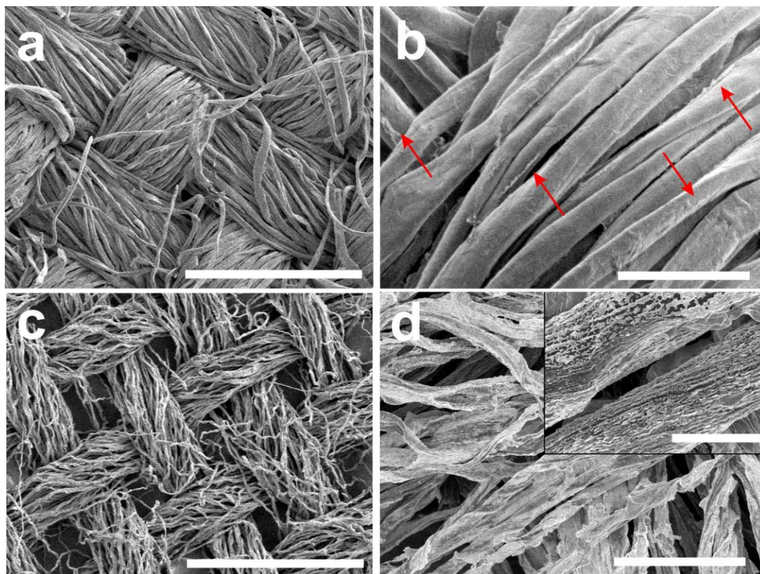
Supplementary Figure S1. SEM images of the CMC60MTM40-1% coated fabric. (a-d) Surface of CMC60MTM40-1%, (a,b) before burning, and (c,d,inset) after burning. The arrows guide the eye to locate rougher areas of the conformal coating of individual fibers (a,c, scale bar 500 \mu\text{m} ; b,d, scale bar 50 \mu\text{m} , inset of d, scale bar 5 \mu\text{m} ).
