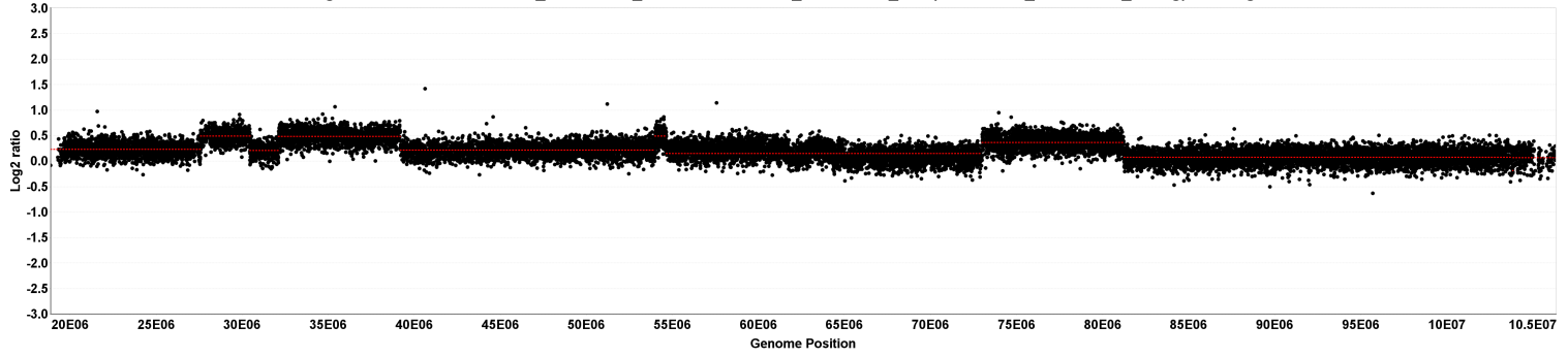
chr15 segmentation for 529552A02_2013-06-20_532 vs. 529552A02_2013-06-20_635 (529552A02_2013-06-20_unavg) - 8 segments
