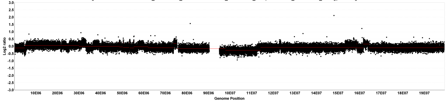
chr4 segmentation for 529552A02_2013-06-20_532 vs. 529552A02_2013-06-20_635 (529552A02_2013-06-20_unavg) - 7 segments
