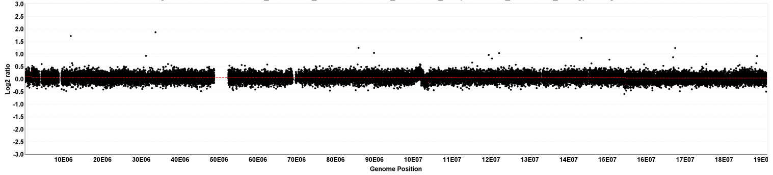
chr5 segmentation for 529552A02_2013-06-20_532 vs. 529552A02_2013-06-20_635 (529552A02_2013-06-20_unavg) - 15 segments
