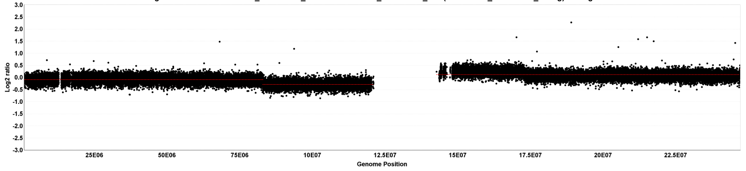
chr2 segmentation for 529552A02_2013-06-20_532 vs. 529552A02_2013-06-20_635 (529552A02_2013-06-20_unavg) - 9 segments
