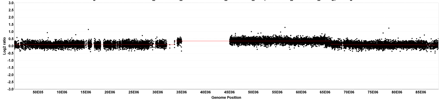
chr17 segmentation for 529552A02_2013-06-20_532 vs. 529552A02_2013-06-20_635 (529552A02_2013-06-20_unavg) - 5 segments
