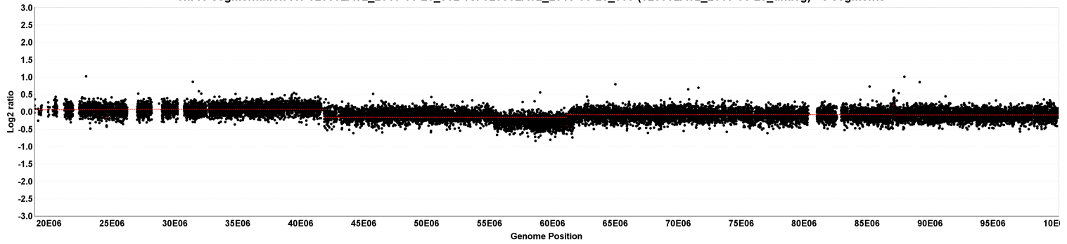
chr15 segmentation for 529552A02_2013-06-20_532 vs. 529552A02_2013-06-20_635 (529552A02_2013-06-20_unavg) - 8 segments
