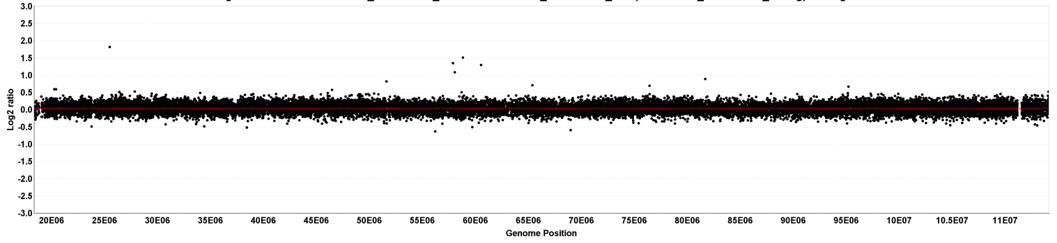
chr14 segmentation for 529552A02_2013-06-20_532 vs. 529552A02_2013-06-20_635 (529552A02_2013-06-20_unavg) - 11 segments
