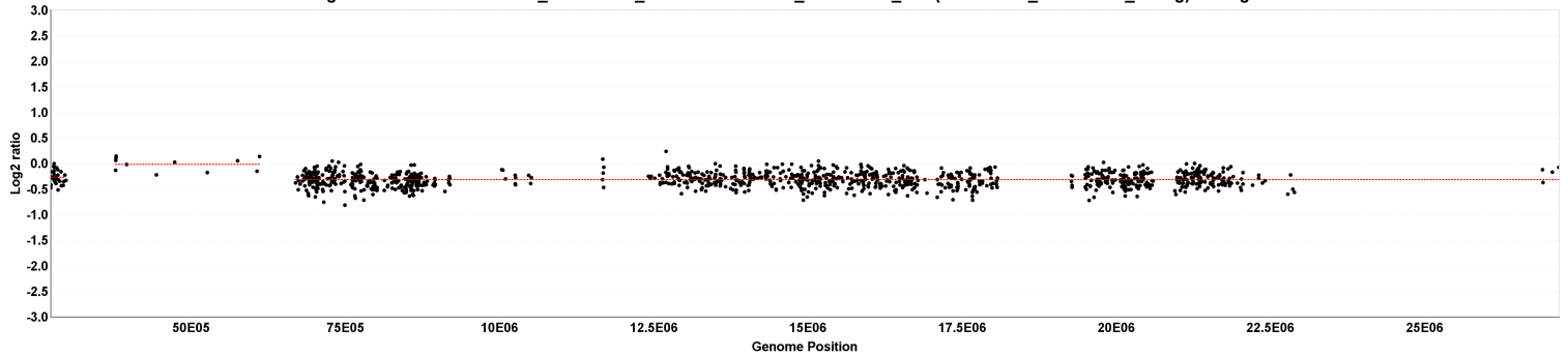
chrY segmentation for 529552A02_2013-06-20_532 vs. 529552A02_2013-06-20_635 (529552A02_2013-06-20_unavg) - 3 segments
