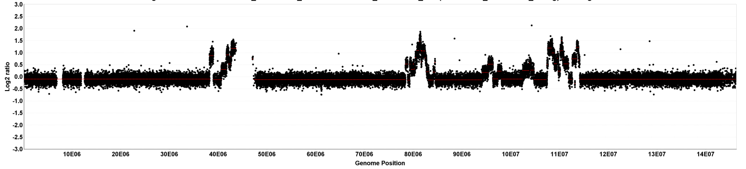
chr9 segmentation for 529552A02_2013-06-20_532 vs. 529552A02_2013-06-20_635 (529552A02_2013-06-20_unavg) - 5 segments
