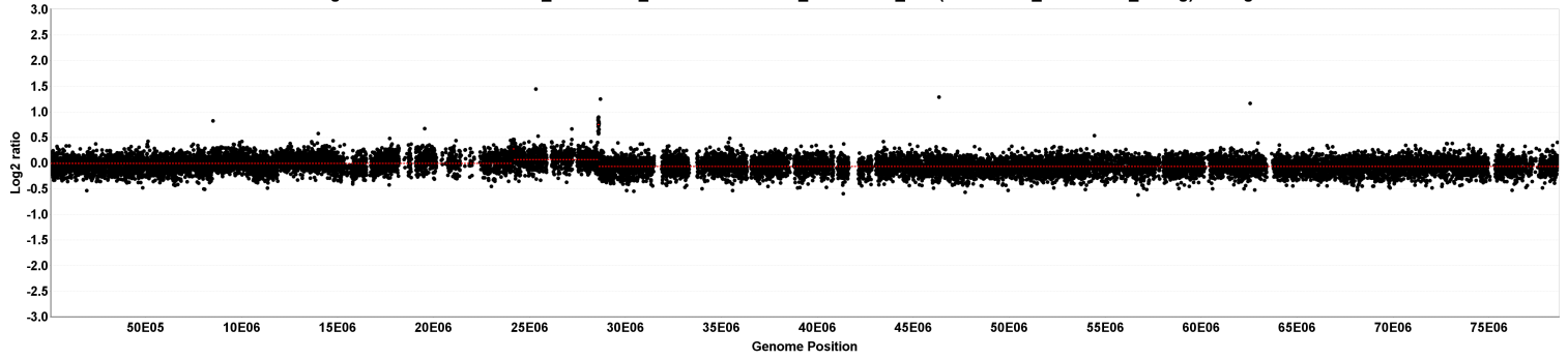
chr18 segmentation for 529552A02_2013-06-20_532 vs. 529552A02_2013-06-20_635 (529552A02_2013-06-20_unavg) - 1 segment
