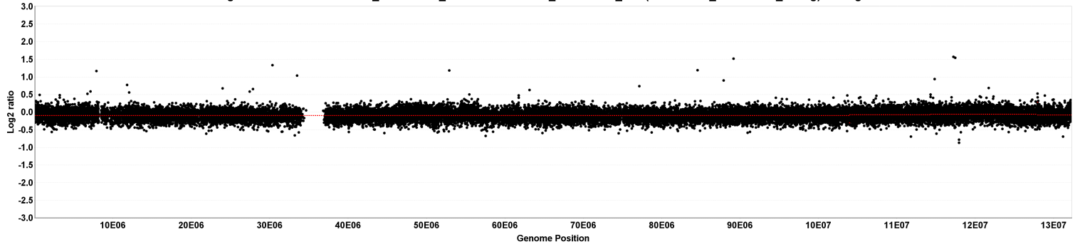
chr13 segmentation for 529552A02_2013-06-20_532 vs. 529552A02_2013-06-20_635 (529552A02_2013-06-20_unavg) - 1 segment
