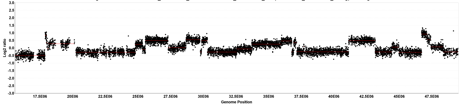
chrX segmentation for 529552A02_2013-06-20_532 vs. 529552A02_2013-06-20_635 (529552A02_2013-06-20_unavg) - 8 segments
