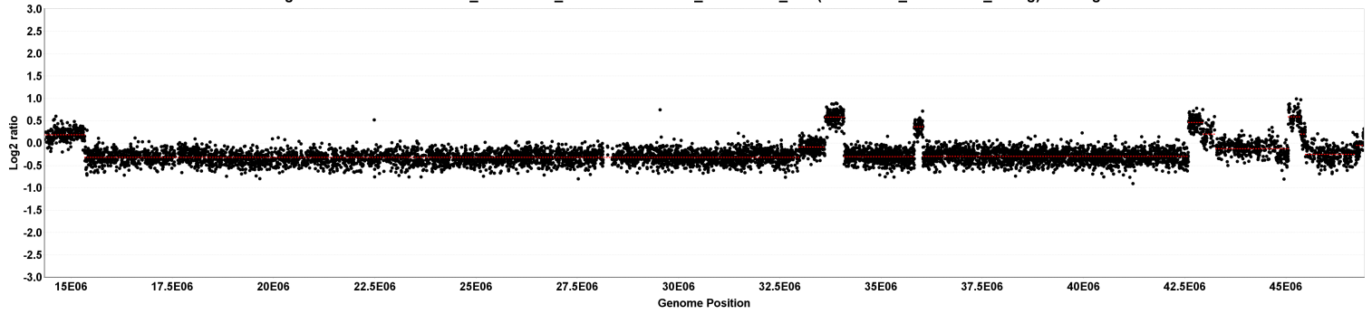
chr22 segmentation for 529552A02_2013-06-20_532 vs. 529552A02_2013-06-20_635 (529552A02_2013-06-20_unavg) - 30 segments
