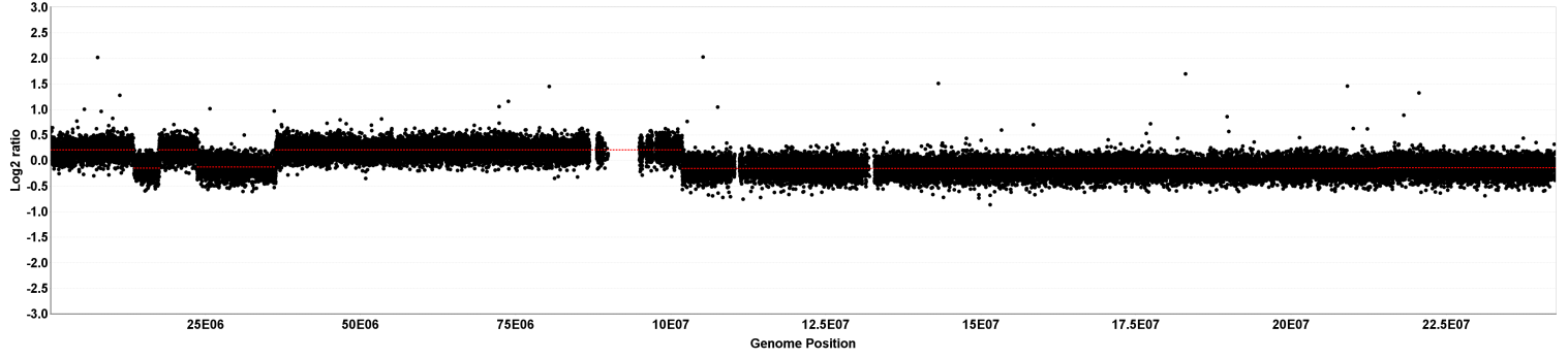
chr3 segmentation for 529552A02_2013-06-20_532 vs. 529552A02_2013-06-20_635 (529552A02_2013-06-20_unavg) - 26 segments
