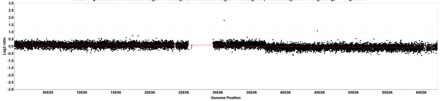
chr20 segmentation for 529552A02_2013-06-20_532 vs. 529552A02_2013-06-20_635 (529552A02_2013-06-20_unavg) - 9 segments
