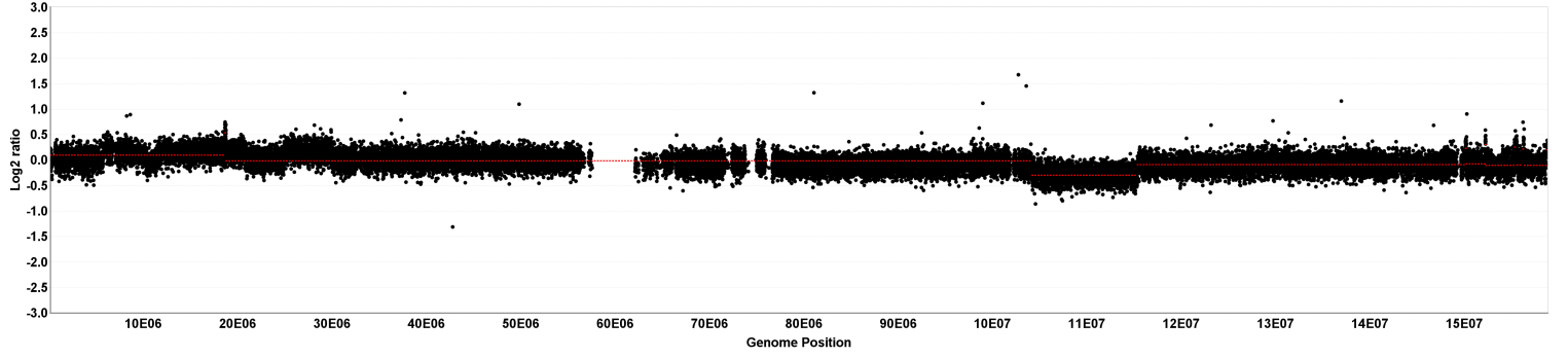
chr8 segmentation for 529552A02_2013-06-20_532 vs. 529552A02_2013-06-20_635 (529552A02_2013-06-20_unavg) - 55 segments
