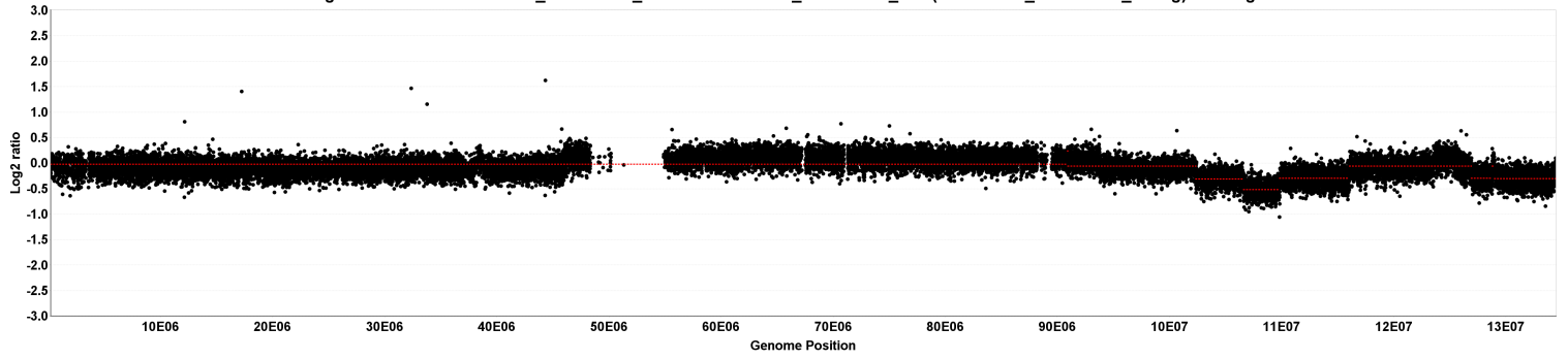
chr12 segmentation for 529552A02_2013-06-20_532 vs. 529552A02_2013-06-20_635 (529552A02_2013-06-20_unavg) - 7 segments
