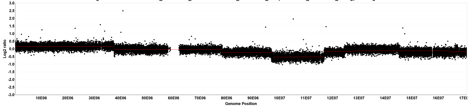
chr7 segmentation for 529552A02_2013-06-20_532 vs. 529552A02_2013-06-20_635 (529552A02_2013-06-20_unavg) - 14 segments
