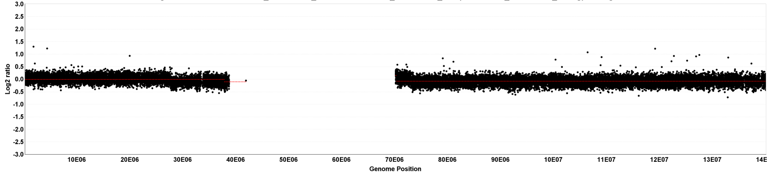
chr10 segmentation for 529552A02_2013-06-20_532 vs. 529552A02_2013-06-20_635 (529552A02_2013-06-20_unavg) - 13 segments
