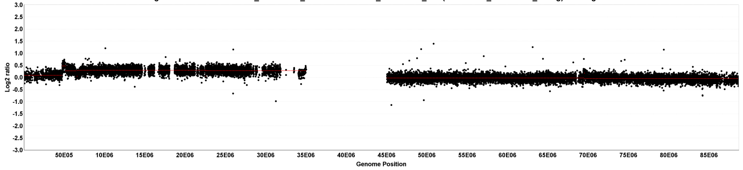
chr17 segmentation for 529564A02_2012-12-19_532 vs. 529564A02_2012-12-19_635 (529564A02_2012-12-19_unavg) - 21 segments
