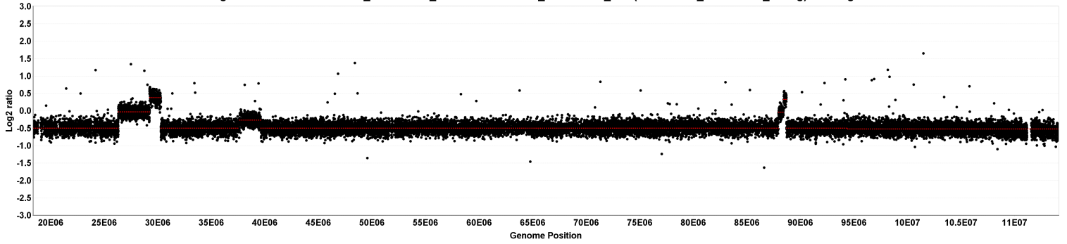
chr14 segmentation for 529564A02_2012-12-19_532 vs. 529564A02_2012-12-19_635 (529564A02_2012-12-19_unavg) - 7 segments
