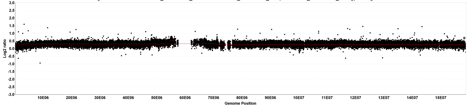
chr8 segmentation for 529564A02_2012-12-19_532 vs. 529564A02_2012-12-19_635 (529564A02_2012-12-19_unavg) - 7 segments
