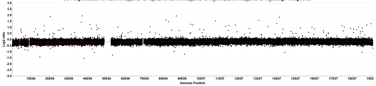
chr5 segmentation for 529564A02_2012-12-19_532 vs. 529564A02_2012-12-19_635 (529564A02_2012-12-19_unavg) - 12 segments
