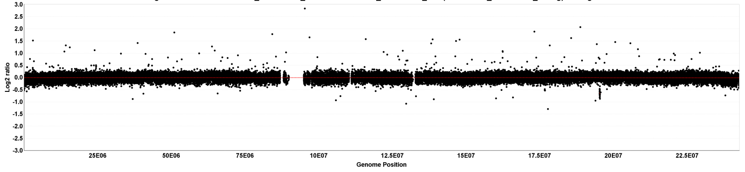
chr3 segmentation for 529564A02_2012-12-19_532 vs. 529564A02_2012-12-19_635 (529564A02_2012-12-19_unavg) - 3 segments
