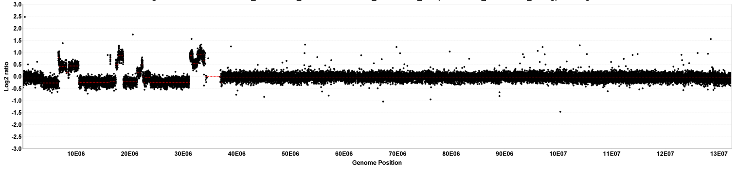
chr13 segmentation for 529564A02_2012-12-19_532 vs. 529564A02_2012-12-19_635 (529564A02_2012-12-19_unavg) - 11 segments
