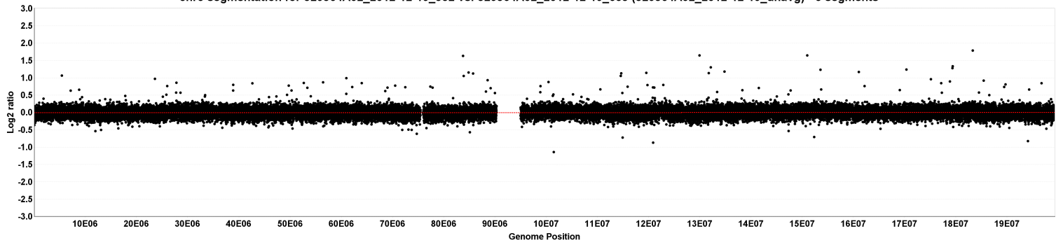
chr4 segmentation for 529564A02_2012-12-19_532 vs. 529564A02_2012-12-19_635 (529564A02_2012-12-19_unavg) - 5 segments
