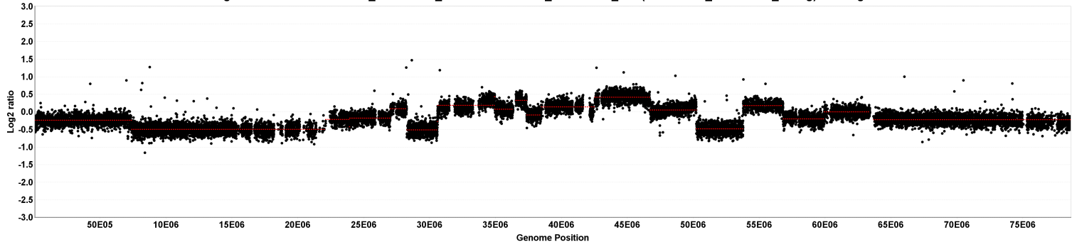
chr18 segmentation for 529564A02_2012-12-19_532 vs. 529564A02_2012-12-19_635 (529564A02_2012-12-19_unavg) - 8 segments
