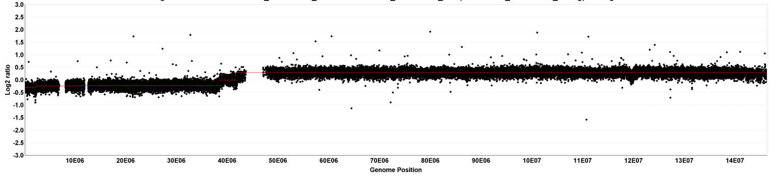
chr9 segmentation for 529564A02_2012-12-19_532 vs. 529564A02_2012-12-19_635 (529564A02_2012-12-19_unavg) - 5 segments
