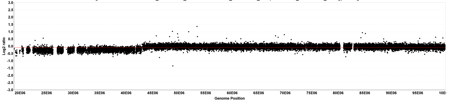
chr15 segmentation for 529564A02_2012-12-19_532 vs. 529564A02_2012-12-19_635 (529564A02_2012-12-19_unavg) - 1 segment
