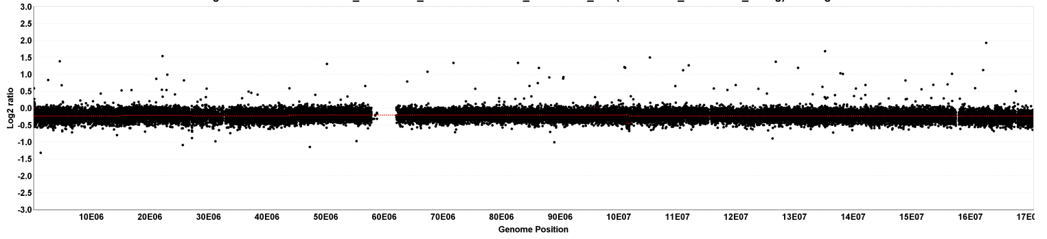
chr7 segmentation for 529564A02_2012-12-19_532 vs. 529564A02_2012-12-19_635 (529564A02_2012-12-19_unavg) - 5 segments
