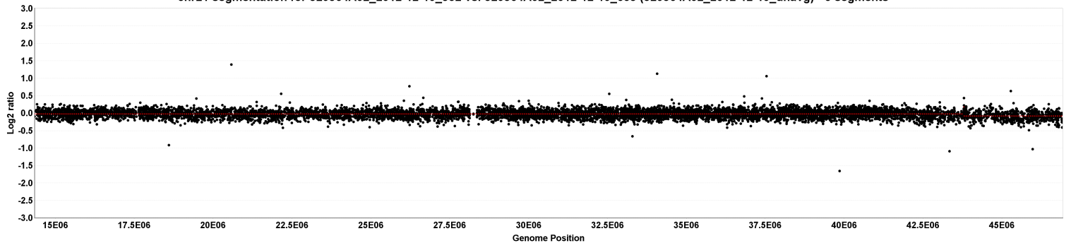
chr22 segmentation for 529564A02_2012-12-19_532 vs. 529564A02_2012-12-19_635 (529564A02_2012-12-19_unavg) - 5 segments
