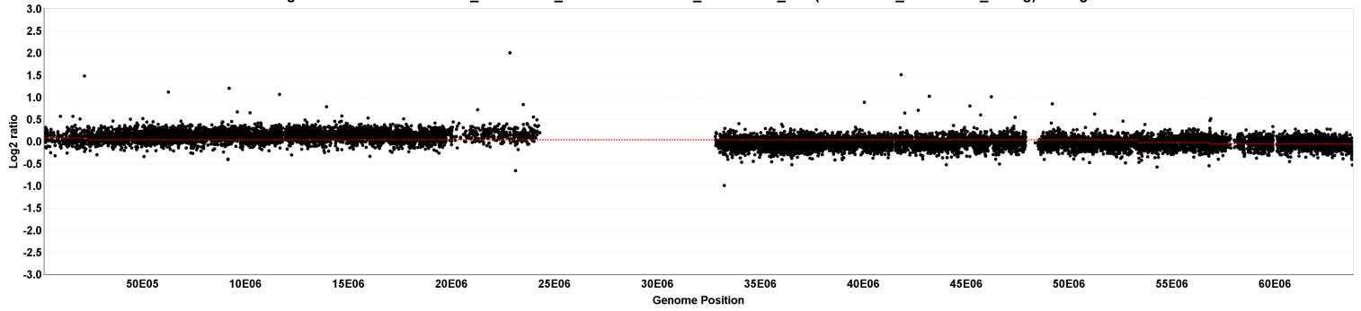
chr20 segmentation for 529564A02_2012-12-19_532 vs. 529564A02_2012-12-19_635 (529564A02_2012-12-19_unavg) - 3 segments
