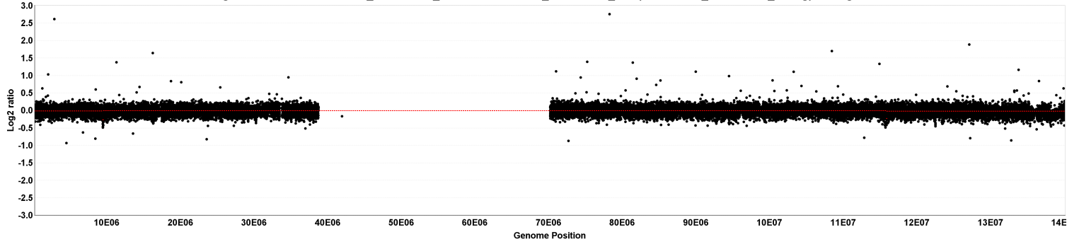
chr10 segmentation for 529564A02_2012-12-19_532 vs. 529564A02_2012-12-19_635 (529564A02_2012-12-19_unavg) - 9 segments
