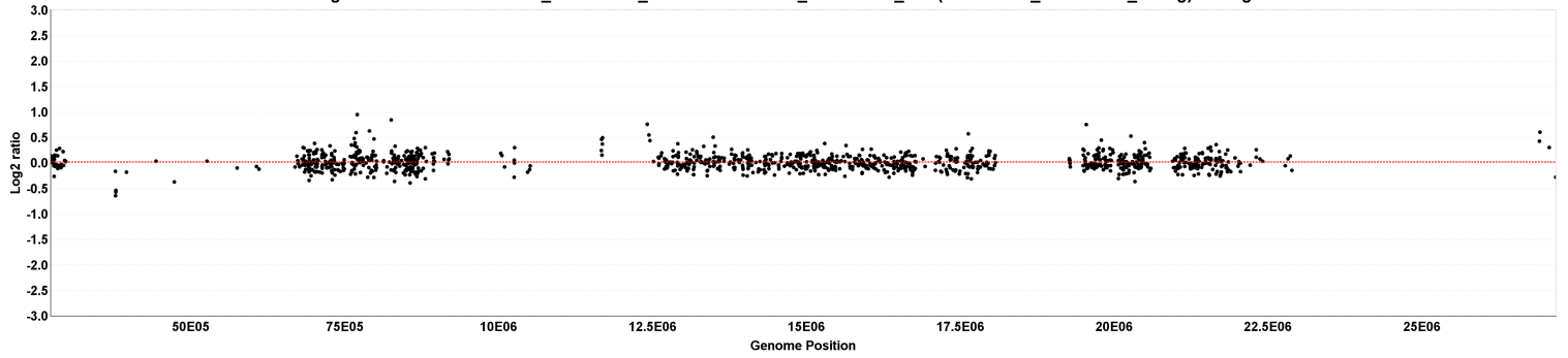
chrY segmentation for 529564A02_2012-12-19_532 vs. 529564A02_2012-12-19_635 (529564A02_2012-12-19_unavg) - 1 segment
