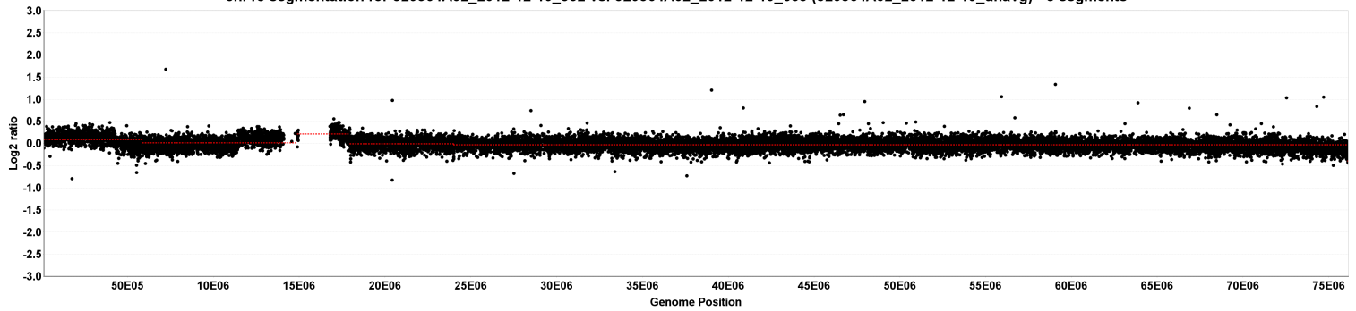
chr19 segmentation for 529564A02_2012-12-19_532 vs. 529564A02_2012-12-19_635 (529564A02_2012-12-19_unavg) - 7 segments
