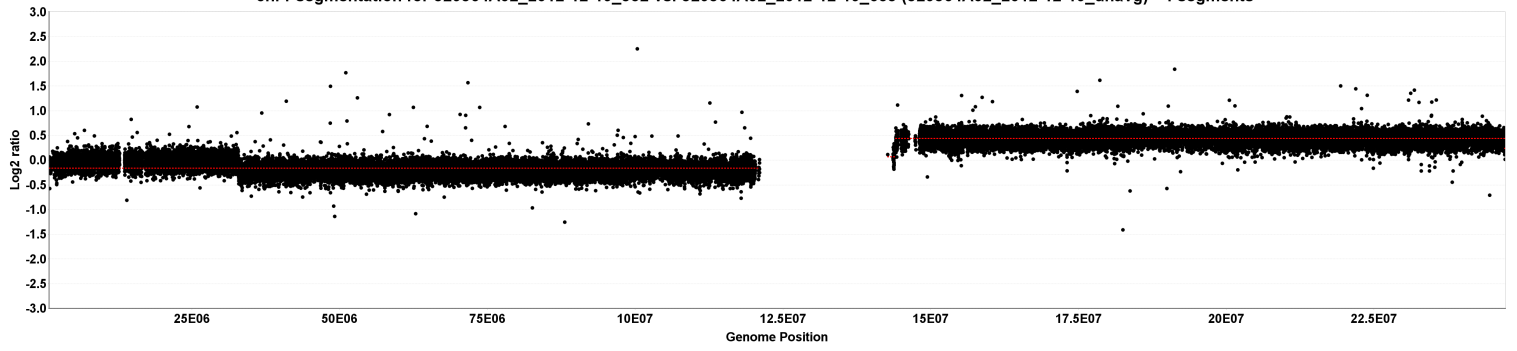
chr2 segmentation for 529564A02_2012-12-19_532 vs. 529564A02_2012-12-19_635 (529564A02_2012-12-19_unavg) - 4 segments
