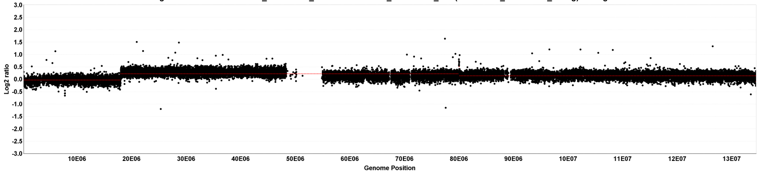
chr12 segmentation for 529564A02_2012-12-19_532 vs. 529564A02_2012-12-19_635 (529564A02_2012-12-19_unavg) - 25 segments
