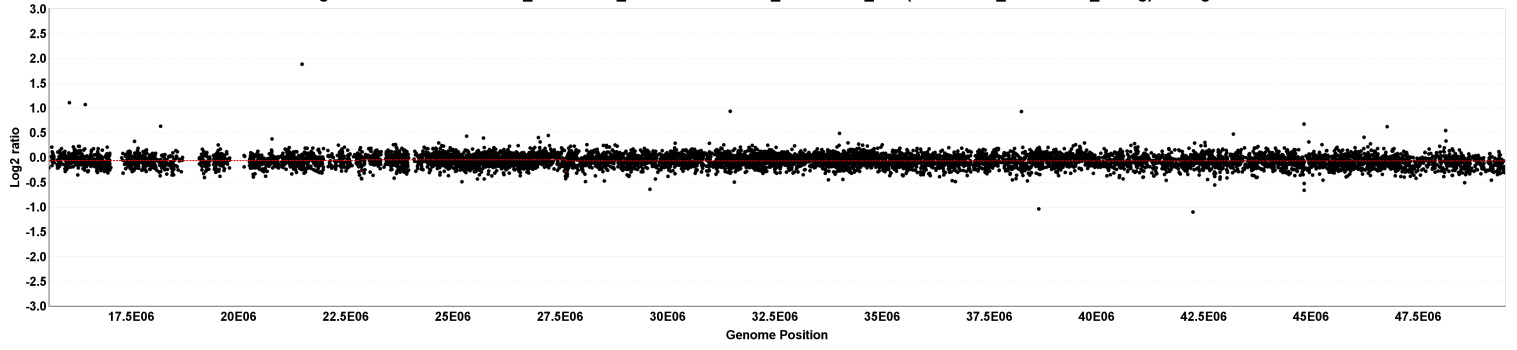
chrX segmentation for 529564A02_2012-12-19_532 vs. 529564A02_2012-12-19_635 (529564A02_2012-12-19_unavg) - 6 segments
